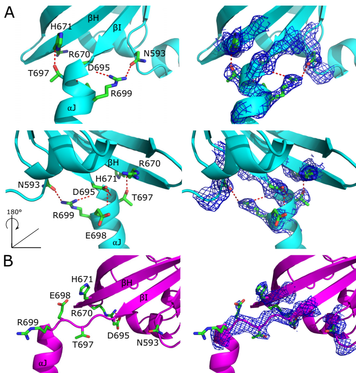
FIG 4 Interaction network around the conserved DIT motif in type I monomers (A) and type II monomers (B) in cartoon and stick representation. Hydrogen bonds are represented with red dashed lines. (Right) Electron densities in that region.
