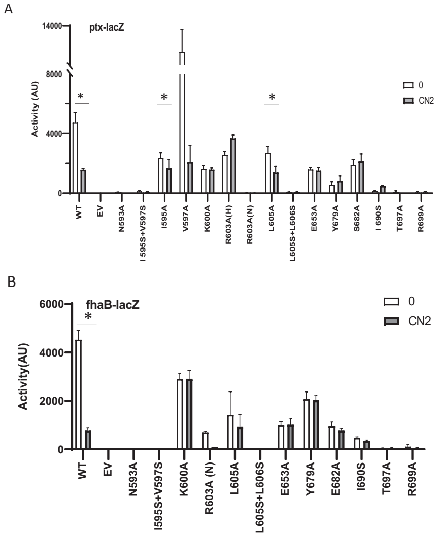
FIG 5 Effect of the substitutions in the PAS domain and its flanking helices on BvgS activity. (A) A ptx-lacZ transcriptional fusion was used to determine the activities of the BvgS variants under standard conditions (0) or after the addition of 2 mM chloronicotinate to the culture medium (CN2) compared to those of wild-type BvgS (WT) and of the strain with an empty vector (EV). The BvgS variants are indicated by the substitution they harbor. For the BvgS R603A variant, hemolytic (H) and nonhemolytic (N) clones were analyzed. (B) A fhaB-lacZ transcriptional fusion was used as described for panel A for the variants that showed no or very little activity with ptx-lacZ . The values are given in arbitrary units, with means and standard deviations. *, statistically significant difference using the nonparametric two-tailed Mann-Whitney test (95% confidence).
