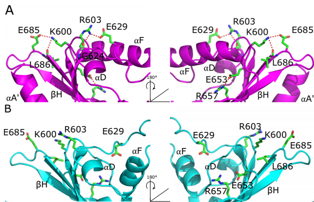
FIG 6 Interaction network in the PAS core domain shown in cartoon and stick representation. The same color code as that of Fig. 4 was used, with type II monomers depicted in pink (A) and type I monomers in blue (B). Hydrogen bonds between side chains are indicated with dashed red lines.
