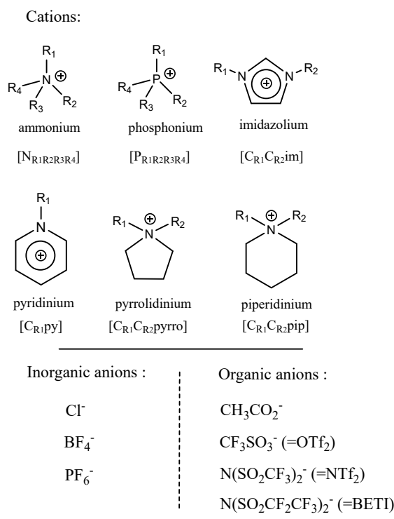
Figure 2. Structures of common cations and anions used in ILs.
