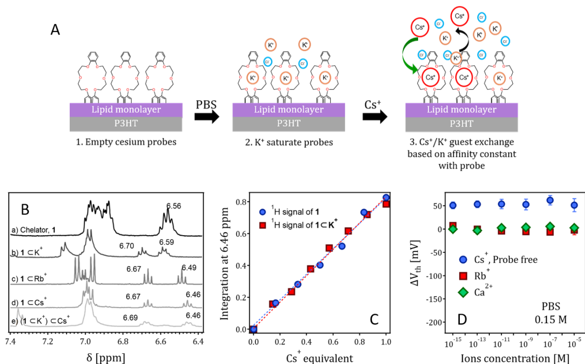
Figure 3: A) Scheme of guest/host exchange mechanism in presence of K^+ competitive ions in solution driven by the greater affinity constant of probe 1 to Cs^+ . B) ^1H RMN spectra of probe 1 in CDCl_3:MeOD:D_2O solution prior to (a) and after K^+ (b), Rb^+ (c), Cs^+ (d) molar equivalent addition. C) Job's plot titration: integrated intensity of the calixarene-related multiplet (6.46 ppm) as a function of Cs^+ concentration in the case of the direct addition of Cs^+ in probe 1 solution (blue circles) or after initial saturation of probe 1 by K^+ (red squares). D) Selectivity measurements: Variation of threshold voltage vs the ions concentration for Rb^+ (red squares) and Ca^{2+} (green diamonds) and for Cs^+ using a sensor with no probes grafted to the lipid layer (blue circles).
