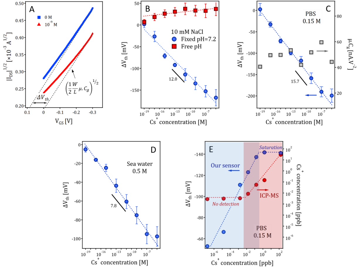
Figure 2: A) Transfer curves obtained in buffered 10 mM NaCl, before (blue) and after (red) exposure of the sensor to 1 nM \text{Cs}^+ ions. The threshold voltage V_{th} is obtained by a linear fitting of the top part of the curves. B-D) Sensor sensitivity in various media: Shift of the threshold voltage \Delta V_{th} as a function of \text{Cs}^+ concentration (in log scale) in non-buffered (red) and pH=7.2 buffered (blue) NaCl solutions (B), in 0.15 M PBS solution (C, blue circles) and in sea water (D). In (B) the grey squares (right Y axis) represent the evolution of the quantity \mu \times C_g (carrier mobility \times dielectric capacitance) inferred from the slope of the transfer curves. Note the variable sensor sensitivity (slope) in the different media: 12 mV/decade in pH=7.2 buffer NaCl, 15.7 mV/decade in 0.15 M PBS and 7.8 mV/decade in sea water. E) Comparison of the performances of EG-FET sensor (in blue) with ICP-MS based detection (red).
