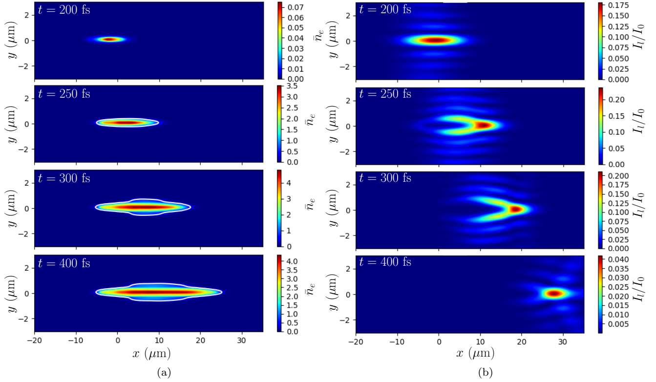
Fig. 2: Spatial and temporal evolutions in the xy plane of the free electron density (a) and laser intensity (b) in silica for 1.3 \mu\text{m} in diameter Bessel–Gauss beam (BG3). The laser pulse comes from the left border and the laser intensity I_l is normalized to the laser peak intensity I_0 = 300 \text{ TW}/\text{cm}^2 . The electron density \bar{n}_e is normalized to n_c = 1.7 \times 10^{21} \text{ cm}^{-3} .
