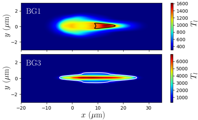
Fig. 3: Final lattice temperature in the xy plane for the BG1 (top panel) and BG3 (bottom panel) with I_0 = 300 TW/cm 2 . The black (for BG1) and white (for BG3) lines correspond to T_l = 1300 K.
