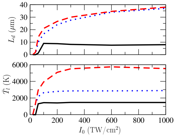
Fig. 4: Evolution of the length of the volume where T_l > T_s (top panel) and of the averaged temperature in this volume (bottom panel) as a function of the peak laser intensity, for BG1 (black solid line), BG2 (blue dotted line) and BG3 (red dashed line) beams.
