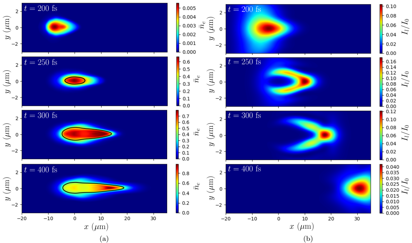
Fig. 1: Spatial and temporal evolutions in the xy plane of the free electron density (a) and laser intensity (b) in silica for 3.11 \mu\text{m} in diameter Bessel–Gauss beam (BG1). The laser pulse comes from the left border and the laser intensity I_t is normalized to the laser peak intensity I_0 = 300 \text{ TW}/\text{cm}^2 . The electron density \bar{n}_e is normalized to n_c = 1.7 \times 10^{21} \text{ cm}^{-3} .
