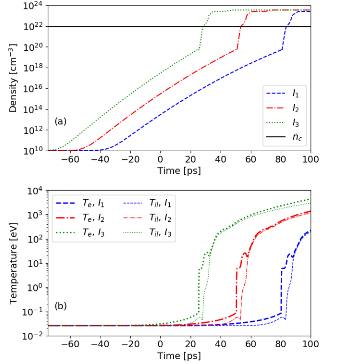
FIG. 3. (a) Evolution of the electron density as a function of time. (b) Evolution of the electron temperature T_e (thick lines) and the ion-lattice temperature T_{il} (thin lines) as a function of time. Simulations are performed with a Gaussian laser shape with a duration of 100 ps for the three following maximum laser intensities I_1 = 10^{13} W.cm ^{-2} , I_2 = 10^{14} W.cm ^{-2} and I_3 = 10^{15} W.cm ^{-2} reached at 200 ps. For the temperatures, solid and dashed lines corresponds to electron and ion-lattice temperatures respectively. The critical density n_c is shown for purpose of comparison.
