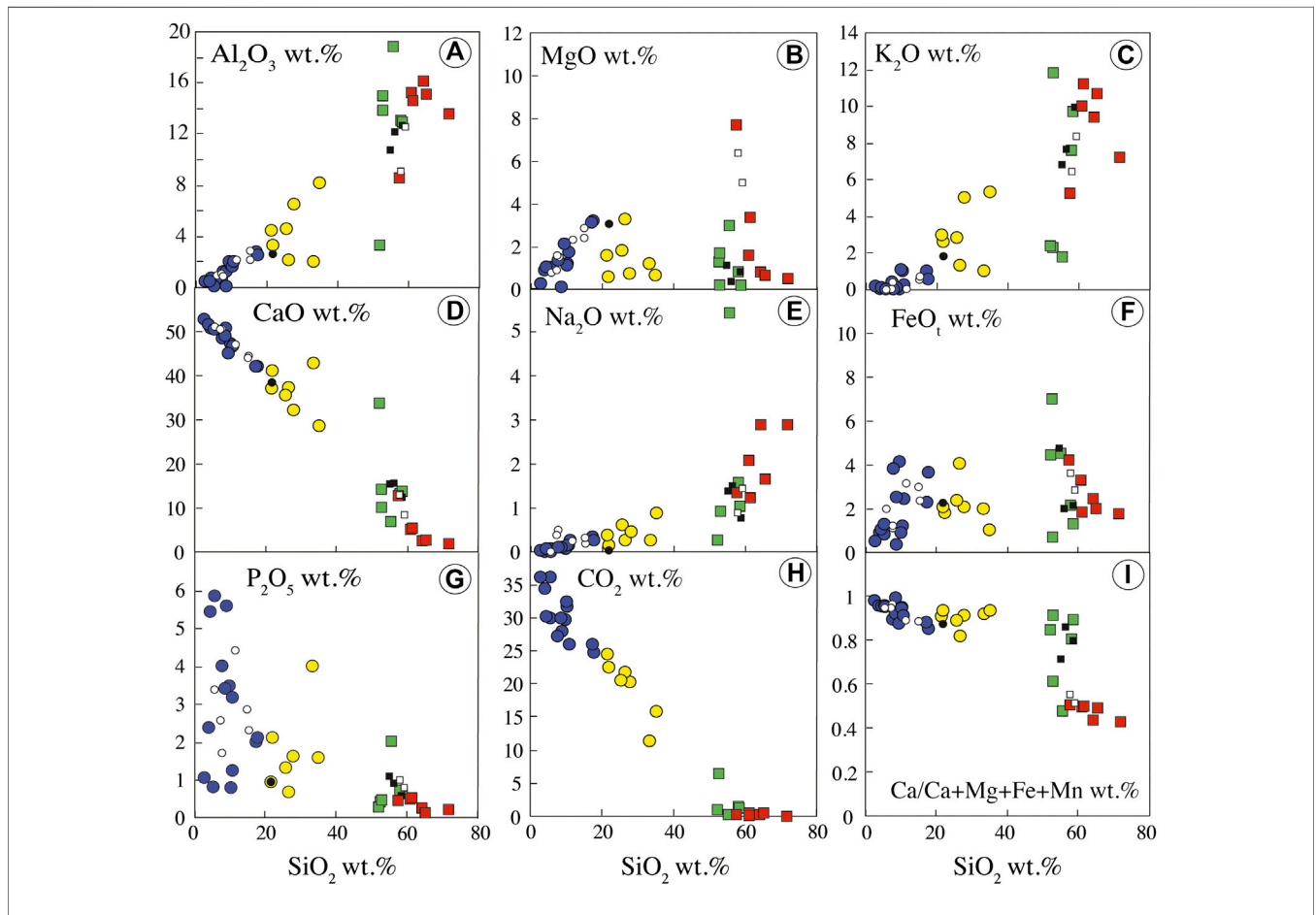
FIGURE 5 | Bulk rock major oxide compositions of the Ihouhaouene carbonatites and syenites. Symbols as in Figure 4 .
