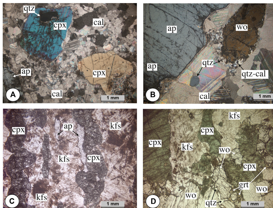
FIGURE 3 | Microphotographs of (A–B) carbonatites and (C–D) syenites. (A) Si-poor brecciated carbonatite with calcite (cal), apatite (ap), and clinopyroxene (cpx) with quartz (qtz) inclusion. (B) Pegmatitic Si-rich carbonatite with apatite and wollastonite (wo) surrounded by quartz (qtz) and calcite. (C) Red syenite with altered K-feldspar (kfs) with apatite and clinopyroxene. (D) White syenite with K-feldspar, clinopyroxene, and wollastonite surrounded by garnet (grt) and quartz.
