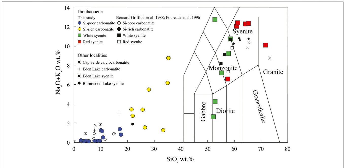
FIGURE 4 | Ihouhouene carbonatites and associated syenites in total alkali-silica (TAS) diagram (after Le Maitre et al., 1989). Cap verde carbonatites (Weinderdorter et al., 2016), Eden Lake carbonatites and syenites (Chakhmouradian et al., 2008), and Burntwood Lake syenites (Martins et al., 2011) are shown.
