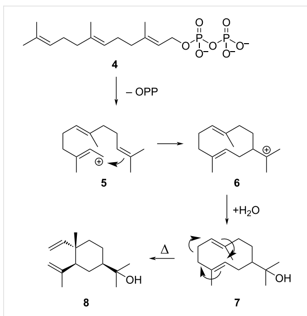
Scheme 2: Biosynthetic formation of hedycaryol (7) and α-elemol (8).
