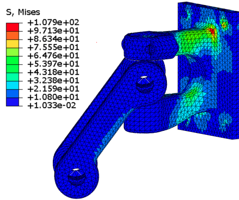
Fig. 7: Iso-chromes of the von Mises equivalent stress for the baseplate of the universal joint pulley
