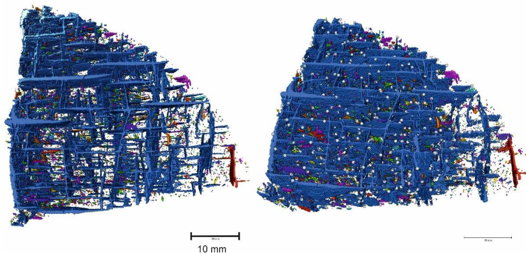
Figure 6. Connectivity pattern of cleat networks after X-ray CT inspection of the sample (resolution: 30 μm). The largest connected cleat array in the sample (resolution of X-ray CT- 30 μm) is shown in blue; other connected cleat volumes are shown in different colors.
