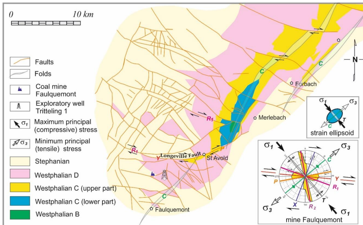
Figure 2. Structural map of the Lorraine Basin supplemented by interpretation fracture patterns in Faulquemont coal mine.
