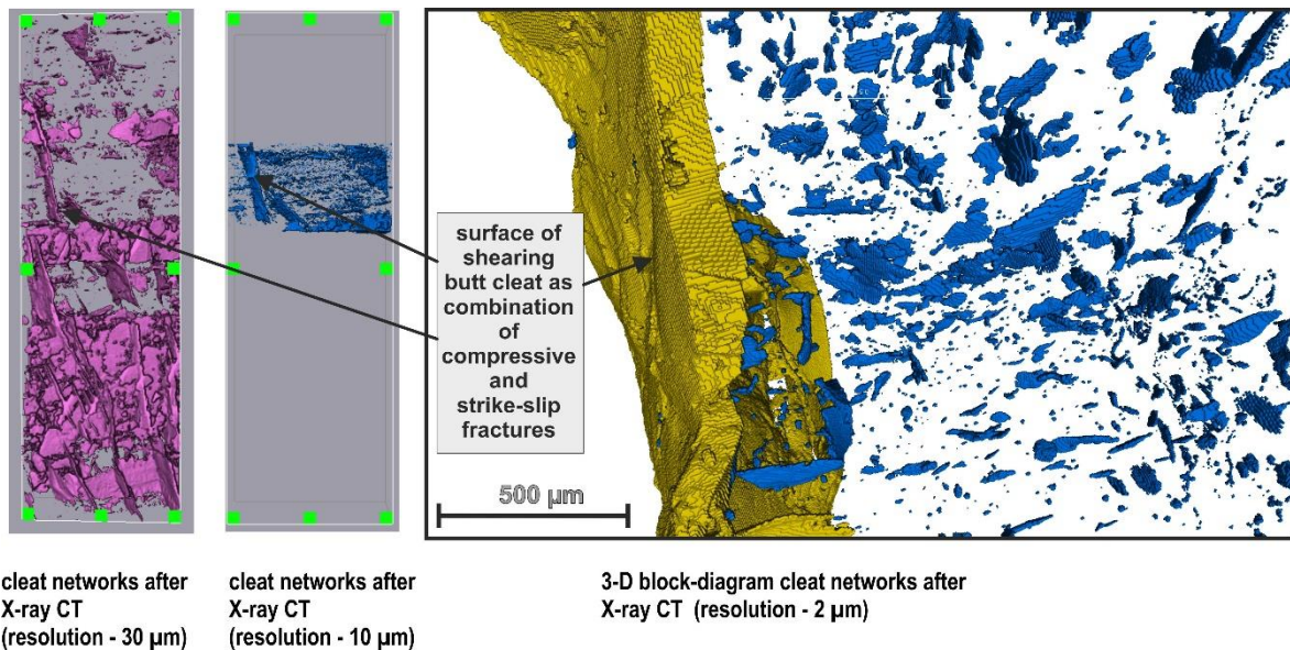
Figure 5. Cleat networks after X-ray CT inspection of the principal specimen and its subvolumes with different resolutions.
