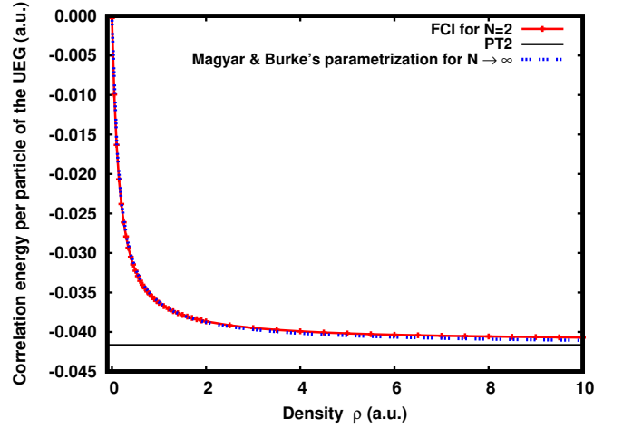
FIG. 3. FCI correlation energy per particle \varepsilon_{\text{c,fUEG}}(\rho) [Eqs. (50) and (52)] of the 1D finite UEG as a function of the density \rho for N = 2 electrons and a plane-wave cutoff n_{\text{max}}^{\text{pw}} = 60 . The exact PT2 correlation energy per particle, which is independent of N and \rho , is indicated as a horizontal line. The correlation energy per particle of the infinite UEG ( N \rightarrow \infty ) as parametrized by Magyar and Burke 24 from essentially numerically exact Bethe-ansatz results is also plotted for comparison.
