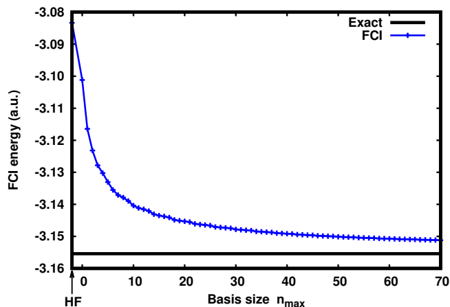
FIG. 1. FCI ground-state energy E_{\text{FCI}}^{\mathcal{B}} [Eq. (10)] of the 1D He-like atom as a function of the basis size n_{\text{max}} . The exact energy is taken from Ref. 24.
