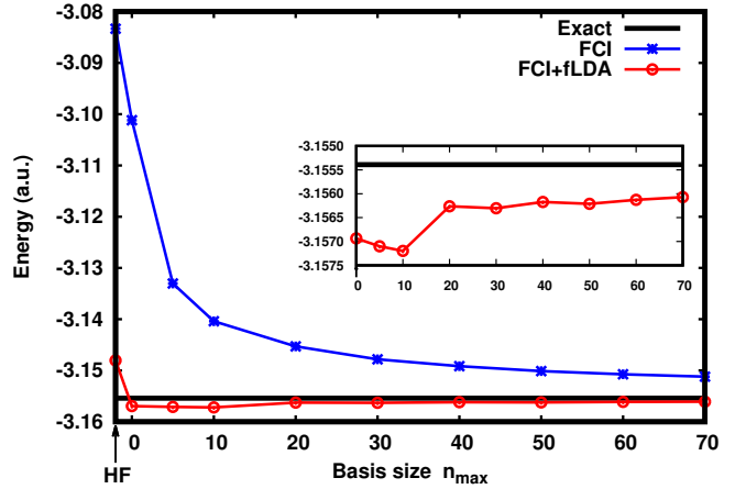
FIG. 7. FCI ground-state energy E_{\text{FCI}}^{\mathcal{B}} [Eq. (10)] and FCI+fLDA ground-state energy E_{\text{FCI+fLDA}}^{\text{w}\mathcal{B}} [Eq. (70)] of the 1D He-like atom as a function of the basis size n_{\max} . The first point labelled by “HF” corresponds to the limiting case where the basis set \mathcal{B} contains only the exact HF occupied orbital (in this case, FCI simply reduces to HF). The exact energy is taken from Ref. 24.
