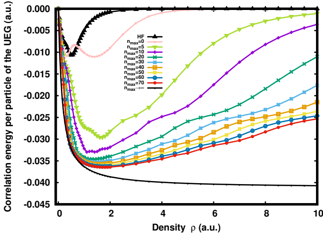
FIG. 5. FCI correlation energy per particle \varepsilon_{c,\text{fUEG}}^{\text{w}\mathcal{B}}(\rho) [Eqs. (66) and (67)] of the 1D finite UEG as a function of the density \rho for N = 2 electrons and for different sizes n_{\max} of the basis set \mathcal{B} of the 1D He-like atom. The curve labelled by “HF” corresponds to the limiting case where the basis set \mathcal{B} contains only the exact HF occupied orbital.
