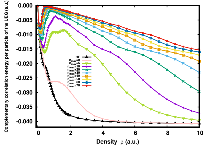
FIG. 6. FCI complementary correlation energy per particle \bar{\varepsilon}_{c,\text{md},\text{fUEG}}^{\text{w}\mathcal{B}}(\rho) [Eq. (68)] of the 1D finite UEG as a function of the density \rho for N = 2 electrons and for different sizes n_{\max} of the basis set \mathcal{B} of the 1D He-like atom. The curve labelled by “HF” corresponds to the limiting case where the basis set \mathcal{B} contains only the exact HF occupied orbital.
