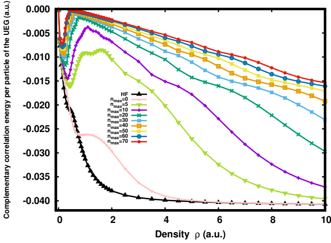
FIG. 6. FCI complementary correlation energy per particle \bar{\varepsilon}_{c,\text{md},\text{fUEG}}^{\text{w}\mathcal{B}}(\rho) [Eq. (70)] of the 1D finite UEG as a function of the density \rho for N = 2 electrons and for different sizes n_{\text{max}} of the basis set \mathcal{B} of the 1D He-like atom. The curve labelled by “HF” corresponds to the limiting case where the basis set \mathcal{B} contains only the exact HF occupied orbital.
