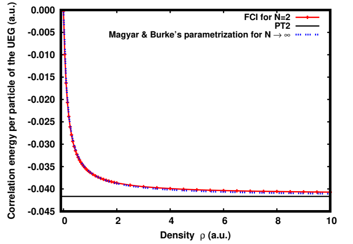
FIG. 3. FCI correlation energy per particle \varepsilon_{\text{c,fUEG}}(\rho) [Eqs. (52) and (54)] of the 1D finite UEG as a function of the density \rho for N = 2 electrons and a plane-wave cutoff n_{\text{max}}^{\text{pw}} = 60 . The exact PT2 correlation energy per particle, which is independent of N and \rho , is indicated as a horizontal line. The correlation energy per particle of the infinite UEG ( N \rightarrow \infty ) as parametrized by Magyar and Burke 19 from essentially numerically exact Bethe-ansatz results is also plotted for comparison.
