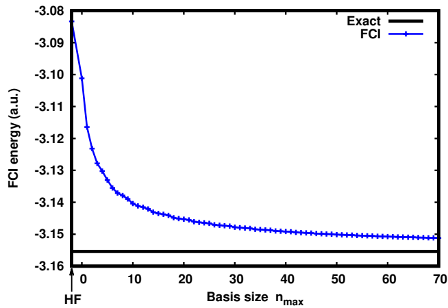
FIG. 1. FCI ground-state energy E_{\text{FCI}}^{\mathcal{B}} [Eq. (10)] of the 1D He-like atom as a function of the basis size n_{\text{max}} . The exact energy is taken from Ref. 19.
