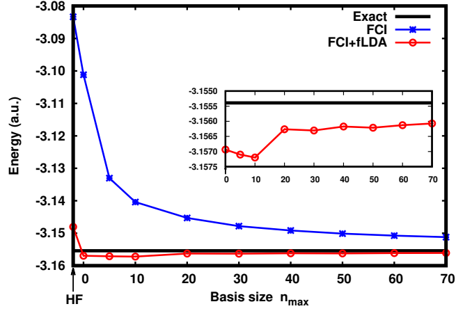
FIG. 7. FCI ground-state energy E_{\text{FCI}}^{\mathcal{B}} [Eq. (10)] and FCI+fLDA ground-state energy E_{\text{FCI+fLDA}}^{\text{w}\mathcal{B}} [Eq. (72)] of the 1D He-like atom as a function of the basis size n_{\text{max}} . The first point labelled by “HF” corresponds to the limiting case where the basis set \mathcal{B} contains only the exact HF occupied orbital (in this case, FCI simply reduces to HF). The exact energy is taken from Ref. 19.
