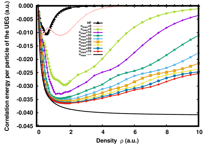
FIG. 5. FCI correlation energy per particle \varepsilon_{\text{c,fUEG}}^{\text{wB}}(\rho) [Eqs. (68) and (69)] of the 1D finite UEG as a function of the density \rho for N = 2 electrons and for different sizes n_{\text{max}} of the basis set \mathcal{B} of the 1D He-like atom. The curve labelled by “HF” corresponds to the limiting case where the basis set \mathcal{B} contains only the exact HF occupied orbital.
