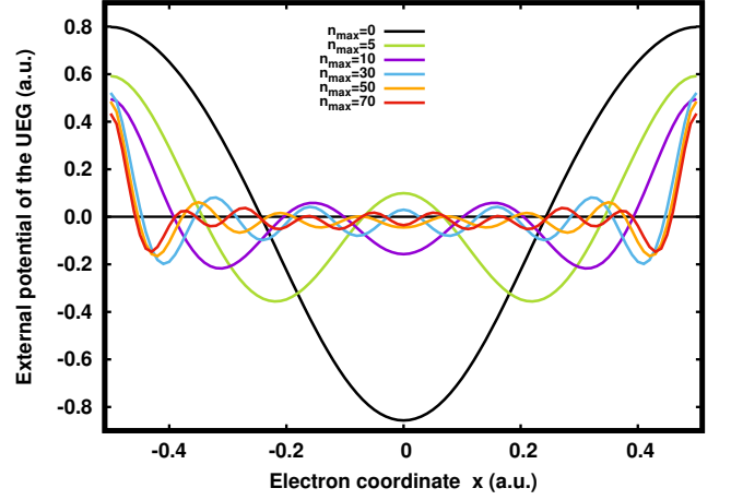
FIG. 4. External optimized potential v^{\text{wB}}(x) [Eq. (63)] keeping a uniform density \rho_0 = 2 a.u. for the 1D finite UEG for N = 2 electrons and for different sizes n_{\text{max}} of the basis set \mathcal{B} of the 1D He-like atom.
