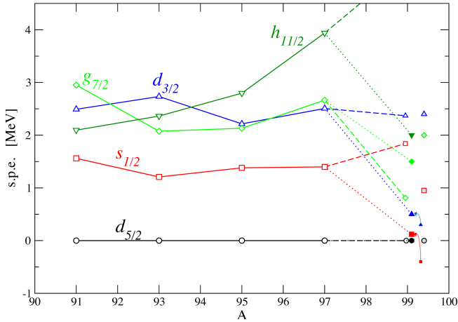
FIG. 1: Neutron SPE for ^{91-99}\text{Zr} isotopes: experiment up to A = 97 [10], and IBFM for ^{99}\text{Zr} : filled symbols, present calculations, arrows showing the modification of values from [2, 9]; open symbols (left) [5]; gray-filled symbols (right) [3, 4]. Note that the SPE of \nu h_{11/2} in our calculations was chosen to reproduce the relative position of the positive- and negative-parity states calculated with the same Hamiltonian.
