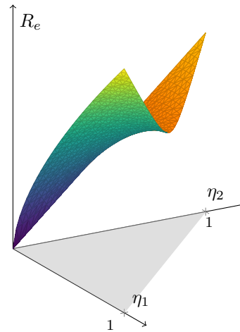
(B) The plan of strategies \eta with cost C_{\text{uni}}(\eta) = 2/3 is represented as a gray surface. The triangulated surface corresponds to the graph of R_e restricted to this set.
