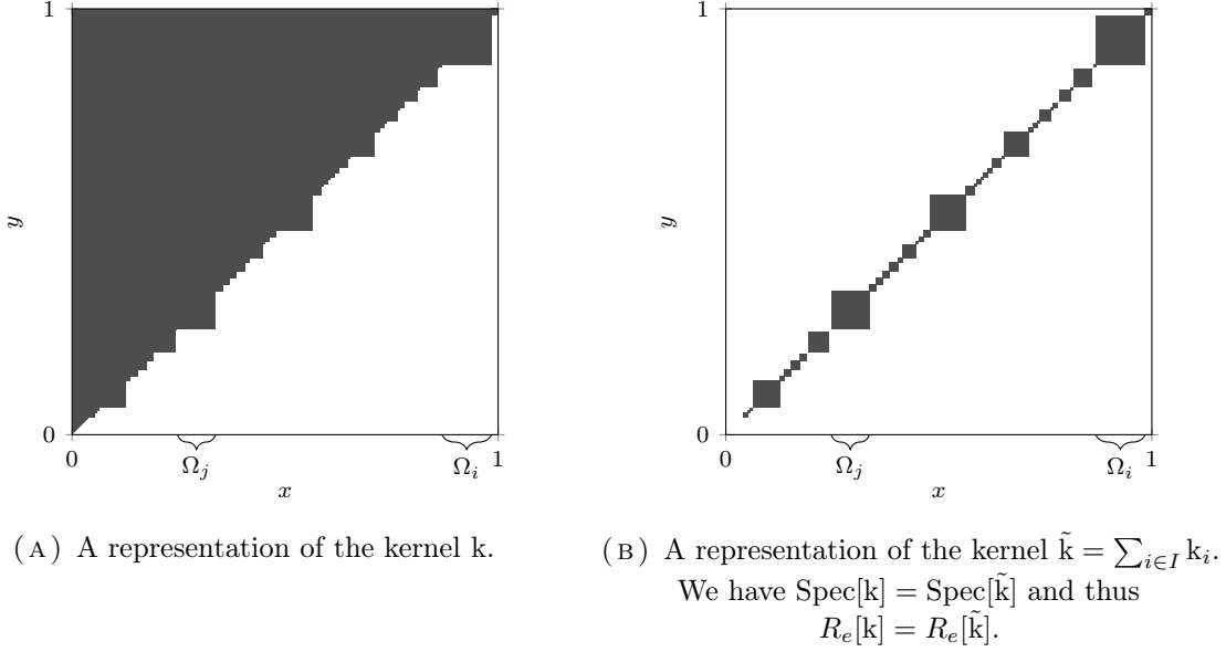
FIGURE 7. Example of a kernel k with the white zone included in \{k = 0\} and the kernel \tilde{k} = \sum_{i \in I} k_i , with k_i = \mathbb{1}_{\Omega_i} k \mathbb{1}_{\Omega_i} and k(\Omega_i, \Omega_j) = 0 for j \prec i .
