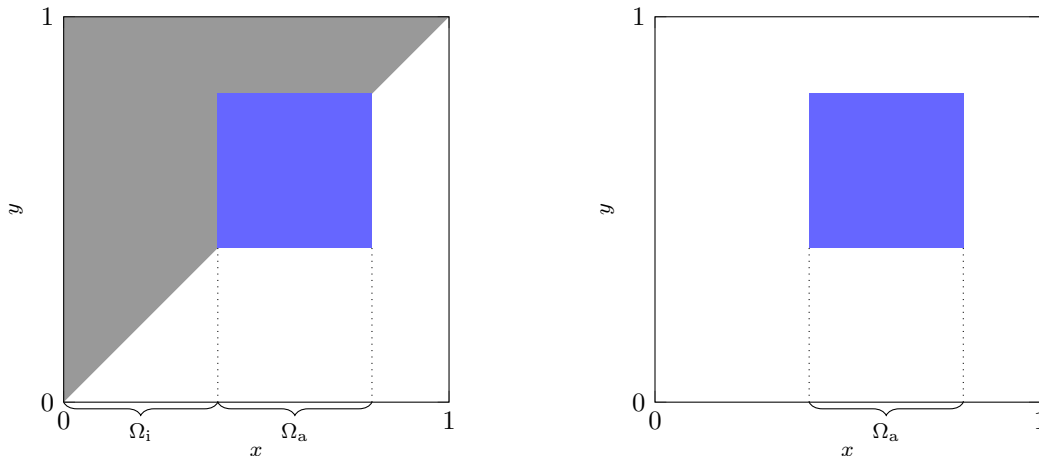
(A) A representation of a monotonic kernel.
