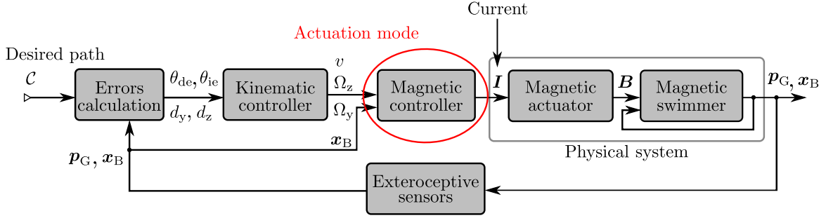
Fig. 3: Block diagram of the 3D path following for any magnetic swimmer robot behaving as a nonholonomic system. In order to change the propulsion mode specific to the swimmer, only the magnetic controller block is adapted.
