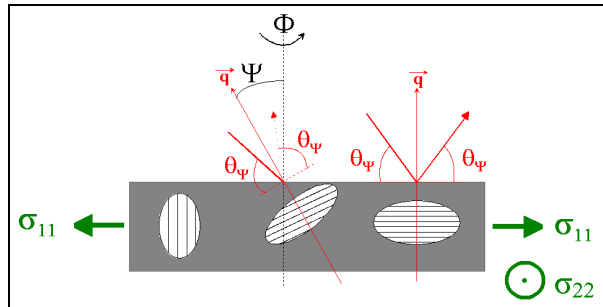
Figure 2: XRD Geometry: \psi is the angle between the surface normal of the sample and the measuring direction, i.e. the normal to the diffracting planes, and \varphi is the azimuth, i.e. the rotation angle around the normal to the sample surface.
