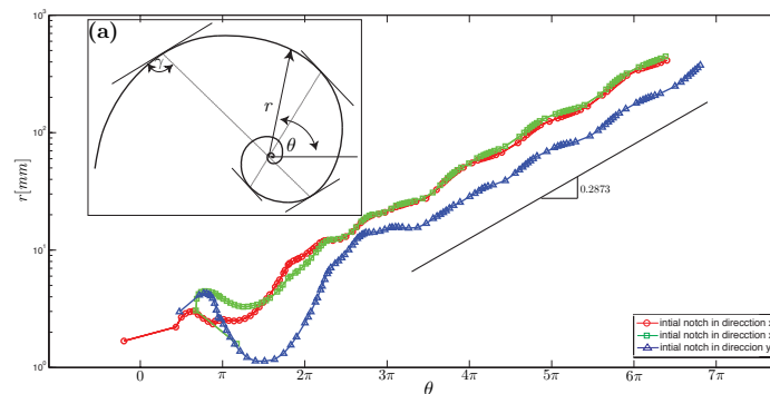
FIGURE 4 – logarithm of distance of points to the center as a function of angle for three different spirals ( \square and \circ : same experimental conditions ; \triangle : initial notch in a perpendicular direction). Inset : geometrical construction used to find the center of the spirals
