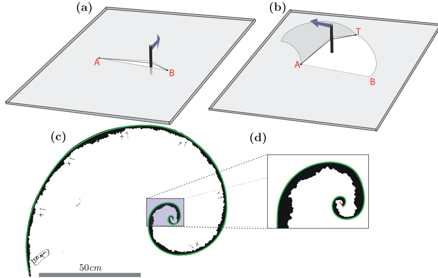
FIGURE 1 – Diagrams of the experiment in initial (a) and intermediate (b) stage. (c) Picture of the final spiral crack path (30 \mu m thickness BOPP sheet). The edge is painted in black for contrast reasons, and a green line is superposed in order to present the path of the crack in the picture. (d) Zoom of the initial part of the spiral, the red line represents the initial notch.
