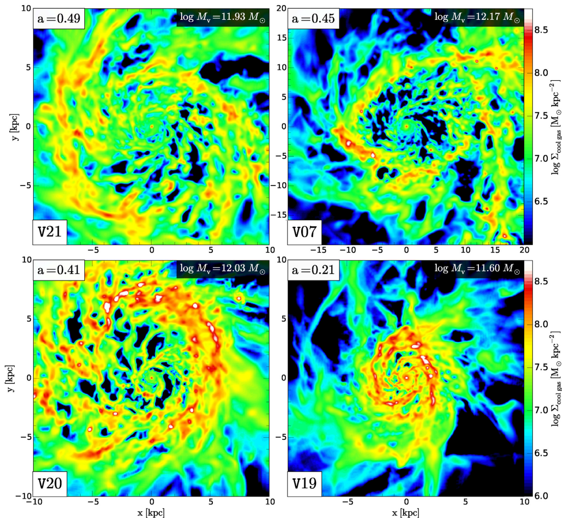
Figure 5. Post-compaction rings. Face-on projected images of gas density in four VELA galaxies at their post-compaction phase, displaying pronounced extended clumpy star-forming rings, fed by cold streams, surrounding gas-depleted central regions. The corresponding stellar density maps show massive compact central bulges.
