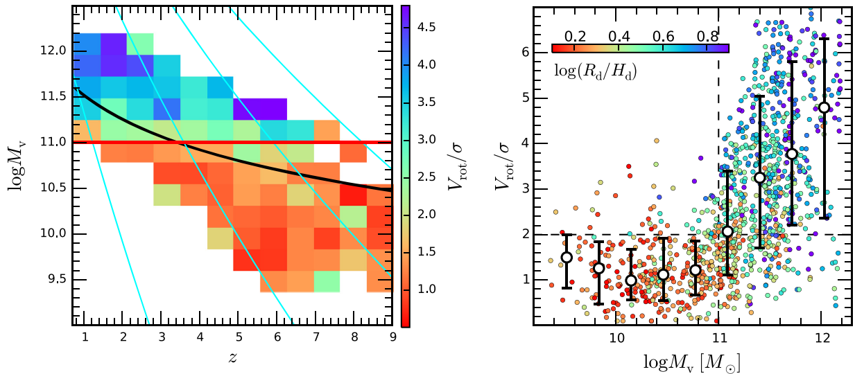
Figure 2. Disc disruption below a characteristic mass. Shown is the degree of disciness in terms of V_{\text{rot}}/\sigma in the VELA simulations. Left: V_{\text{rot}}/\sigma (colour) is averaged within bins in the mass–redshift plane. The black curve refers to the upper limit for effective supernova feedback at a virial velocity V_v = 120 \text{ km s}^{-1} . The cyan curves refer to the Press-Schechter \nu\sigma peaks, for \nu = 1, 2, 3, 4 from left to right, respectively. Right: V_{\text{rot}}/\sigma as a function of halo mass M_v for all the snapshots of all the 34 evolving galaxies. Each point refers to a snapshot, with the median and 1\sigma scatter (16 and 84 percent percentiles) marked in bins of M_v . The colour refers to the alternative measure of disciness by shape using R_d/H_d , showing consistency between the two alternative measures of disciness. In both figures we see a marked transition from non-discs to discs or rings at a threshold mass of M_v \simeq 10^{11} M_\odot , with negligible redshift dependence, as predicted analytically in Dekel et al. (2020).
