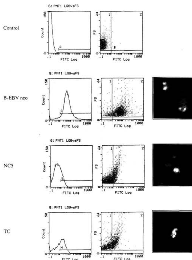
Figure 1. LMP1 immunodetection in EBV-transformed cells. Fluorescence histogram (left) and two-parameter flow cytometry histogram (middle) obtained with control, B-EBV neo, NC5 and TC cell lines. Labeling of the B-EBV neo cell line with an IgG1 secondary antibody was used as a control. LMP1 detection was analyzed by microscopy (right) in these cell types.
