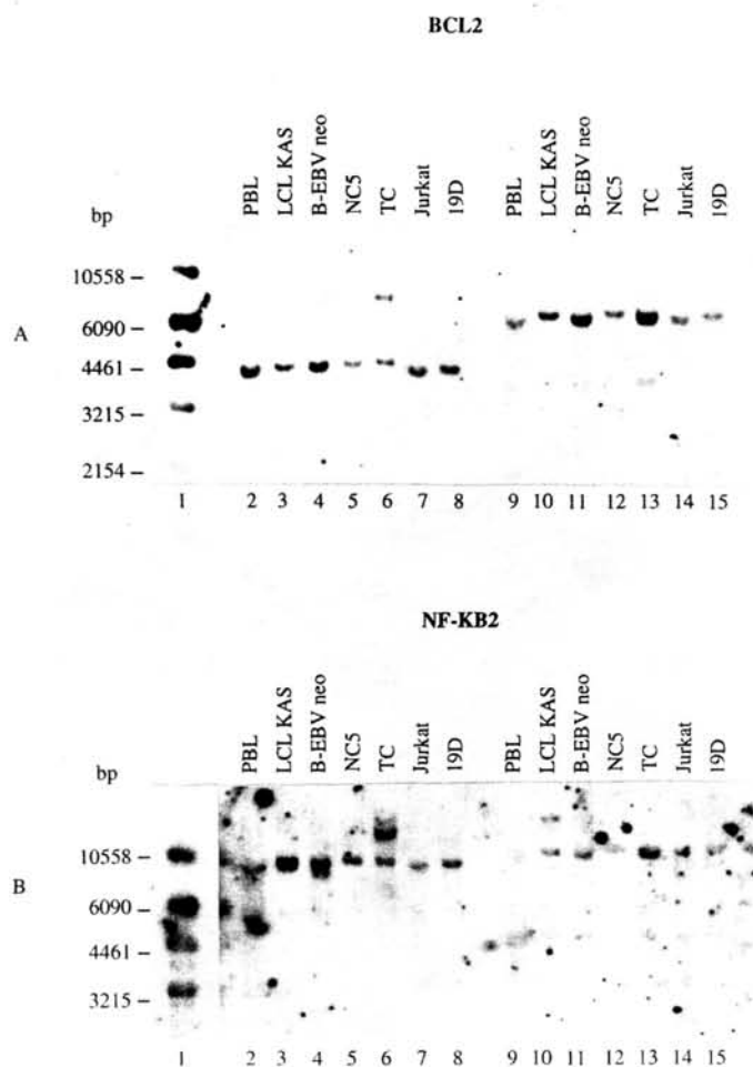
Figure 3. Southern blot analysis of BCL-2 (A) and NF-KB2 (B) genes. DNAs were digested either with BamHI (lanes 2-8) or with HindIII (lanes 9-15). The same blot was used in A and B. The upper band in lane 6 (A and B) results from partial digestion and the upper band in lane 10 (B) seems to result from a polymorphism. Lane 1, molecular weight marker.
