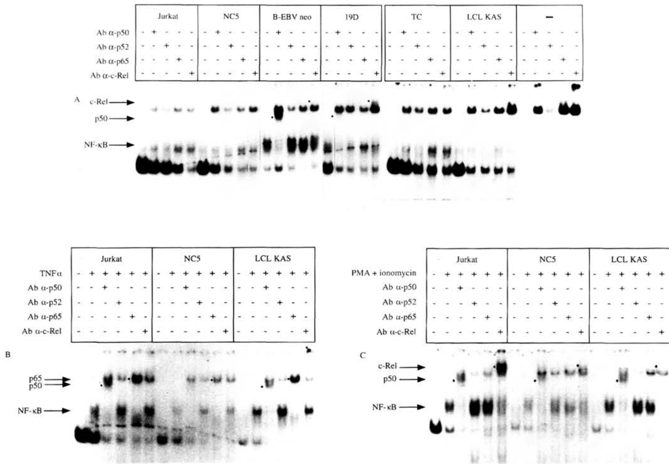
Figure 6. Nuclear extracts were analyzed by band shift experiments with an HIV enhancer \kappa B site probe to study the activation state of NF- \kappa B. Cells were left untreated (A) or activated by TNF \alpha (B) or by PMA + ionomycin (C). Binding of the different antibodies (Ab) to the probe is shown on the right of panel A. The arrows indicate the position of migration of specific DNA-protein complexes. Position of supershifted complexes is indicated with dots.
