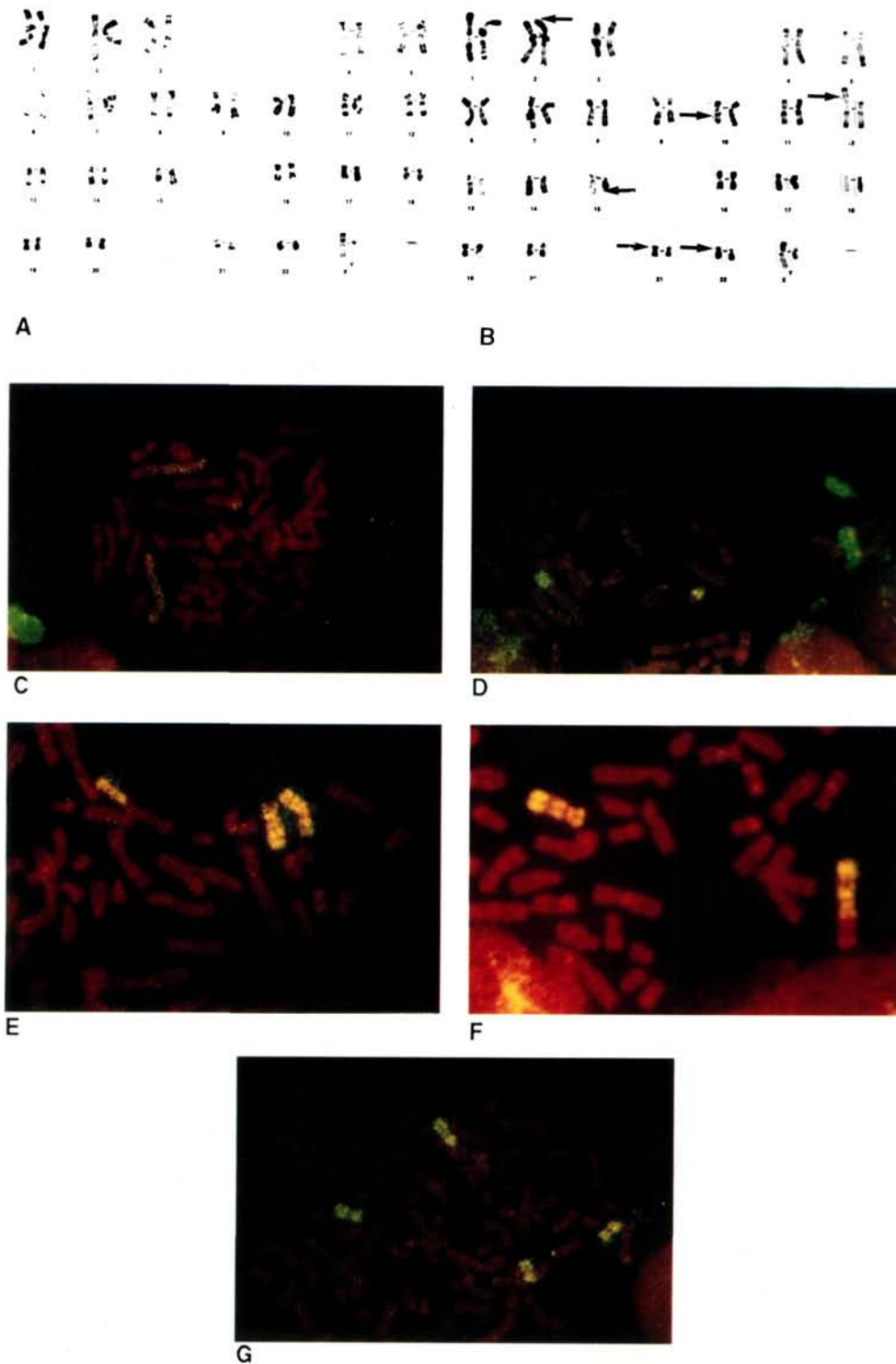
Figure 2. A, Normal R-banded karyotype of a B-EBV neo cell. B, R-banded karyotype of an NC5 cell showing rearrangements. C, D, E, F, G, Metaphase spreads of NC5 cells after hybridization with a painting probe for chromosome 2 (C), 15 (D), 9 (E), 12 (F) and 10 (G). A signal is detected on the distal q arm of rearranged chromosome 15 (C) and on the distal p arm of rearranged chromosome 2 (D). The chromosome 9 signal detected on chromosome 12p reveals a partial 9q trisomy (E). Painting on chromosome 12 confirms the t(9;12) translocation (F). The signal corresponding to the interstitial deletion fragment of chromosome 10 was not found on another metaphase chromosome (E).
