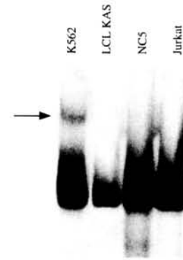
Figure 5. Whole cell extracts were analyzed by band shift experiments with a STAT5-binding site of the bovine \beta casein gene promoter probe to study the activation state of STAT5. The arrow indicates the position of migration of the specific DNA-protein complex.
