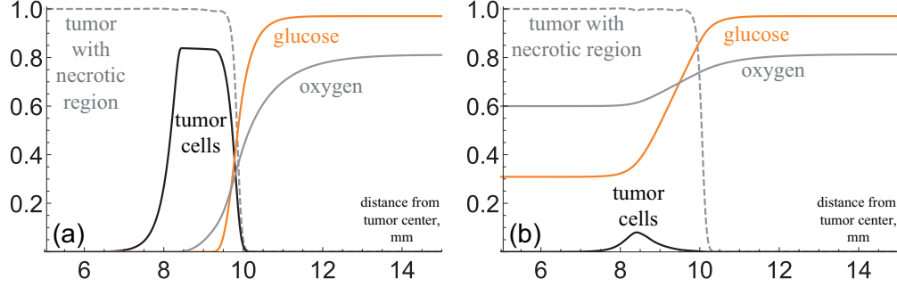
Figure 7: Example of the distributions of model variables in work [244] 1) on the first day of standard radiotherapy, 2) on the ninth day. Black line denotes tumor cells density, gray dashed line – total fraction of alive and dead tumor cells, orange and gray solid lines – levels of glucose and oxygen in tissue.
