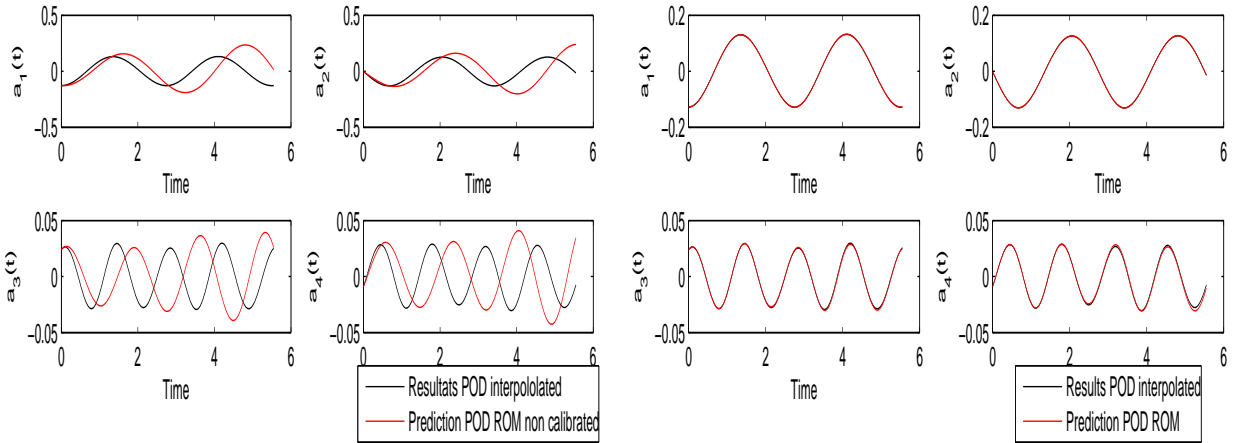
Figure 4: Comparison of the temporal modes before and after calibration ( n = 4 ).
