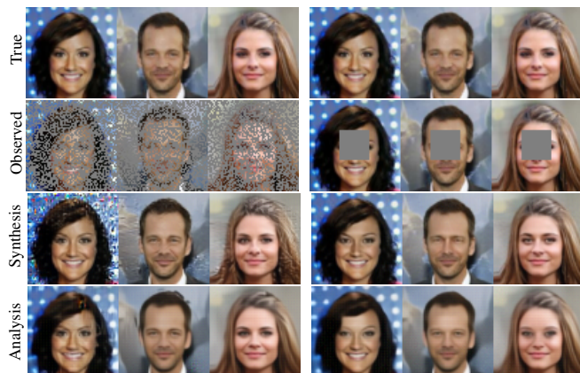
Fig. 2. Inpainting with random mask (left) and structured mask (right), for the same three images of the test set.
