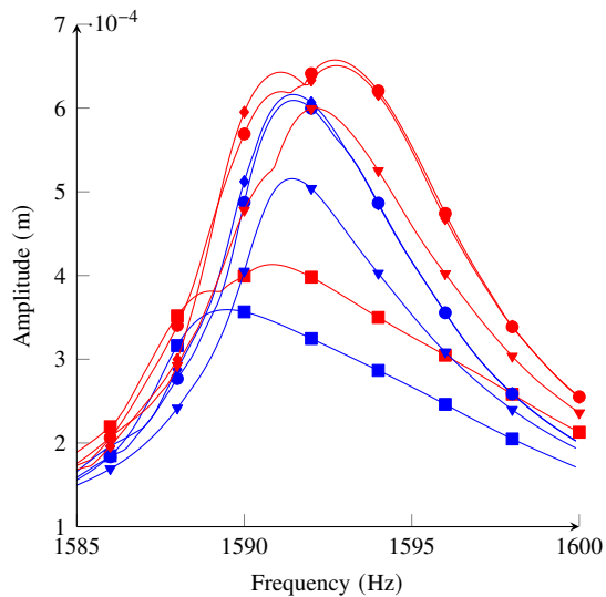
FIGURE 10: FREQUENCY FORCED RESPONSES FOR THE 1F MODE FOR THE SIX BEST STRUCTURES. (—): WITHOUT RANDOM MISTUNING; (—): WITH RANDOM MISTUNING. THE MARKERS (■), (▼), (●), AND (◐) DENOTE THE (A) 24 , (AB) 12 , (2A2B1A1B) 4 AND MP345 SYSTEMS.
