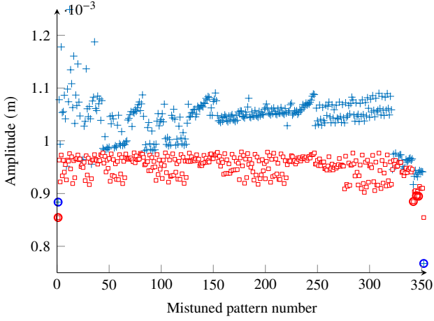
FIGURE 9: MAXIMAL AMPLITUDE DISPLACEMENT FOR THE DIFFERENT MISTUNING PATTERNS FOR THE 1T MODE. (x): COMBINATION OF AB AND BA; (+): COMBINATION OF AA AND BB.
