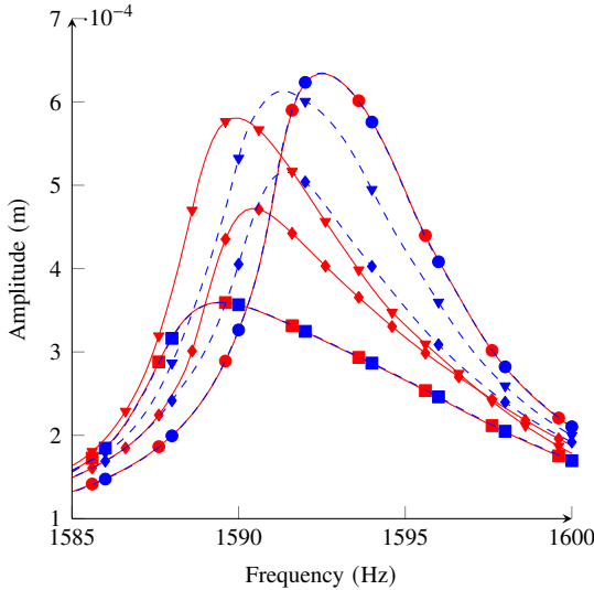
FIGURE 5: FREQUENCY FORCED RESPONSES FOR THE 1F MODE. (—): REFERENCE METHOD; (---): SNCR. THE MARKERS (■), (●), (◆), AND (▼) DENOTE THE (A)_{24} , (B)_{24} , (AB)_{12} , AND (ABBA)_6 STRUCTURES.
