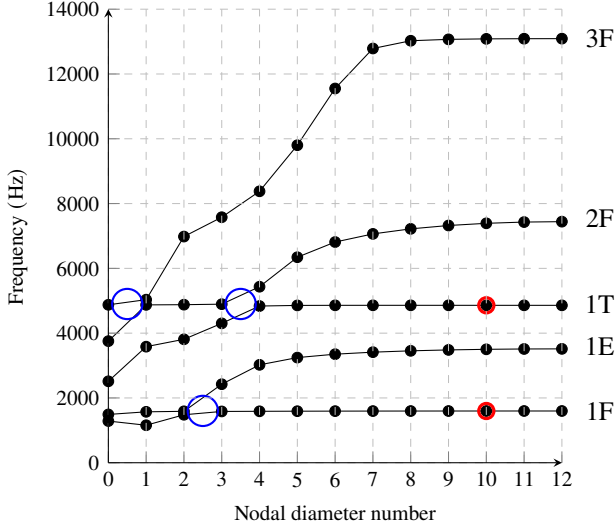
FIGURE 2: NATURAL FREQUENCIES OF EACH NODAL DIAMETER. THE LARGE BLUE CIRCLES DENOTE VEERING AREAS AND SMALL RED CIRCLES DENOTE THE MODES OF INTEREST.
