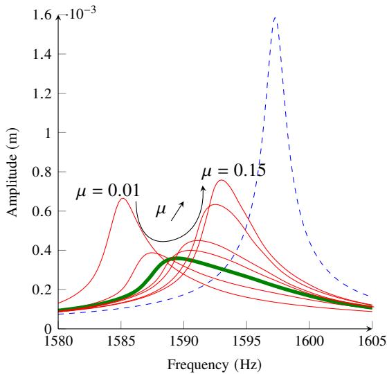
FIGURE 3: FREQUENCY FORCED RESPONSES FOR THE 1F MODE. (- -): LINEAR (STUCK) CASE; (—): OPTIMAL CASE \mu_{1F}^* = 0.03 . (—): OTHER VALUES OF \mu (0.01, 0.02, 0.04, 0.05, 0.1, AND 0.15 IN THIS ORDER).
