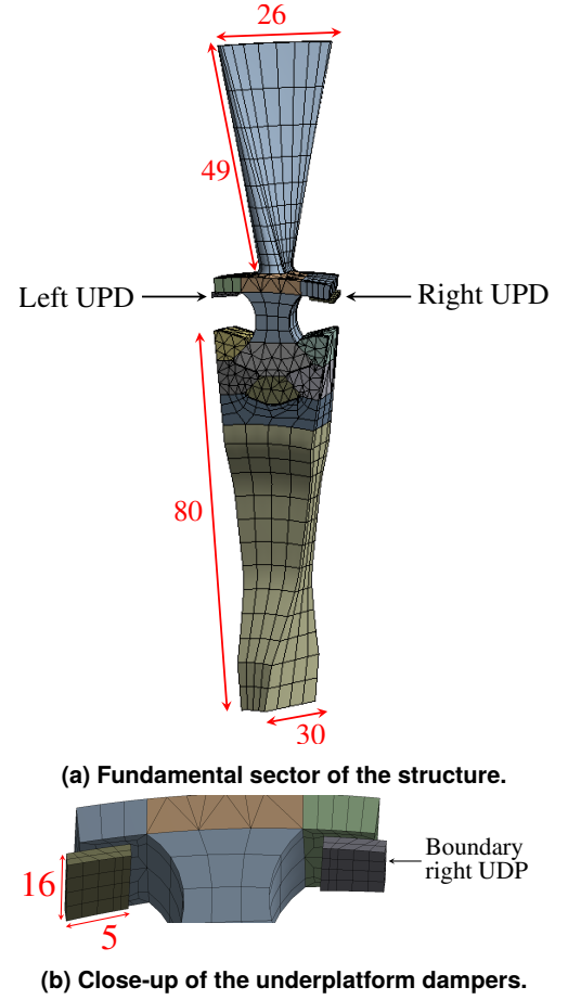
FIGURE 1: DESCRIPTION OF THE MODEL. THE DIMENSIONS ARE IN mm. A PRETWIST ANGLE OF 30^\circ IS APPLIED ON THE BLADE. THE BLADE IS MADE OF ICONEL®738 AND THE DISK OF ICONEL®718.
