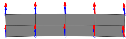
FIGURE 7: ILLUSTRATION OF THE DEFORMED SHAPE OF THE RIGHT UDP BOUNDARY SURFACE FOR THE 1F MODE. DIRECTION AND AMPLITUDE OF THE MAXIMAL DISPLACEMENT FOR: [→] THE (A)_{24} STRUCTURE, AND [→] THE (B)_{24} STRUCTURE.
