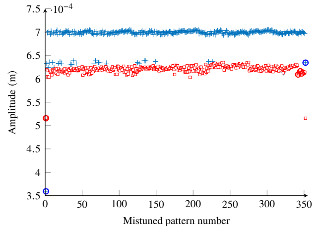
FIGURE 8: MAXIMAL AMPLITUDE DISPLACEMENT FOR THE DIFFERENT MISTUNING PATTERNS FOR THE 1F MODE. (□): COMBINATION OF AB AND BA; (+): COMBINATION OF AA AND BB.
