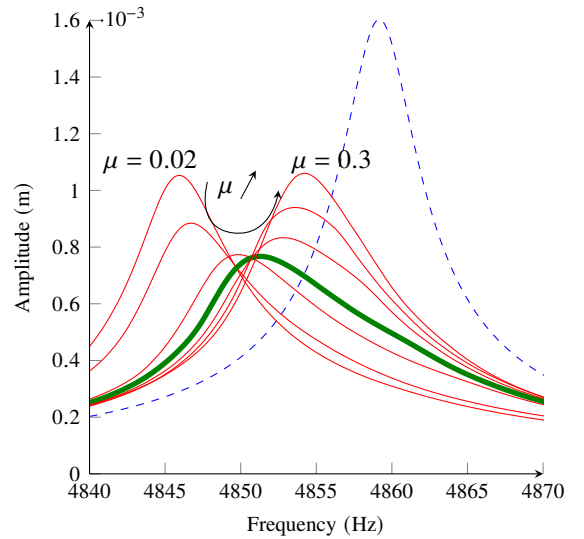
FIGURE 4: FREQUENCY FORCED RESPONSES FOR THE 1T MODE. (- -): LINEAR (STUCK) CASE; (—): OPTIMAL CASE \mu_{1T}^* = 0.1 . (—): OTHERS VALUES OF \mu (0.02, 0.03, 0.07, 0.15, 0.2, AND 0.3 IN THIS ORDER).
