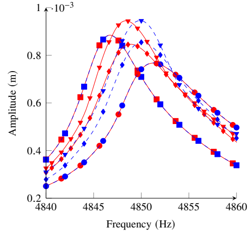
FIGURE 6: FREQUENCY FORCED RESPONSES FOR THE 1T MODE. (—): REFERENCE METHOD; (---): SNCR. THE MARKERS (■), (●), (◆), AND (▼) DENOTE THE (A)_{24} , (B)_{24} , (AB)_{12} , AND (ABBA)_6 STRUCTURES.
