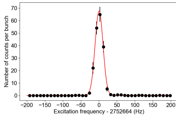
Figure 8: Number of counts/bunch detected on the MCP detector behind the trap as a function of the frequency of the quadrupolar RF excitation. At the resonance frequency \nu_c , ^{39}\text{K}^+ ions are centered in the trap. The gaussian fit to the data, shown in red, has a sigma of 11.0 Hz
