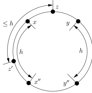
Figure 1: The position placement after h steps (up to symmetry).
