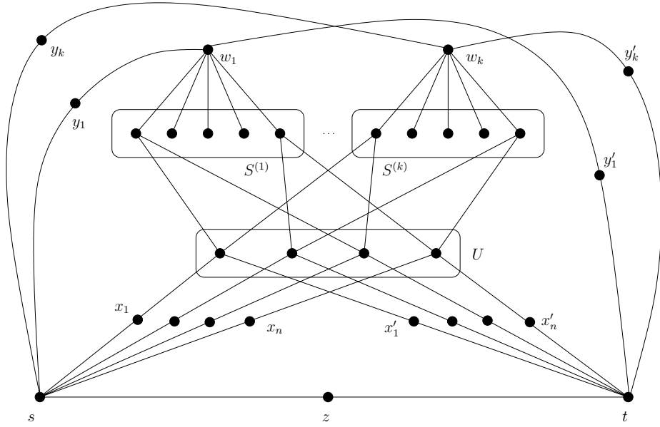
Figure 3: The construction of G .
