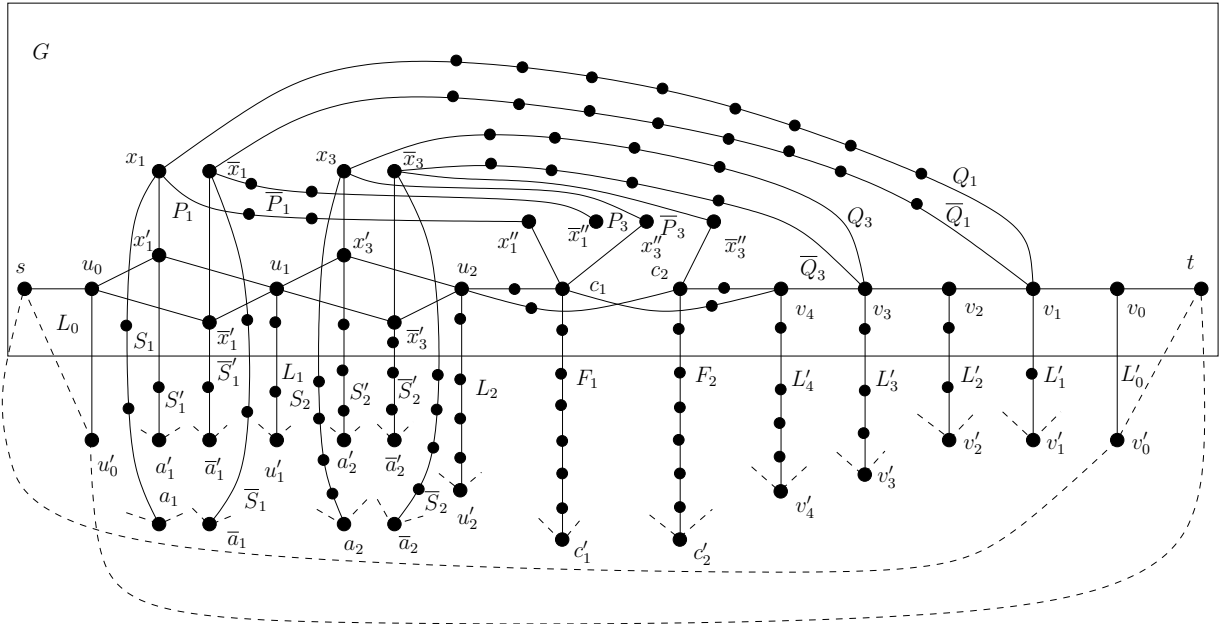
Figure 5: The construction of G' for G shown in Figure 4.
