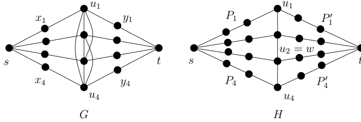
Figure 2: The construction of G and H for p = 4 .
