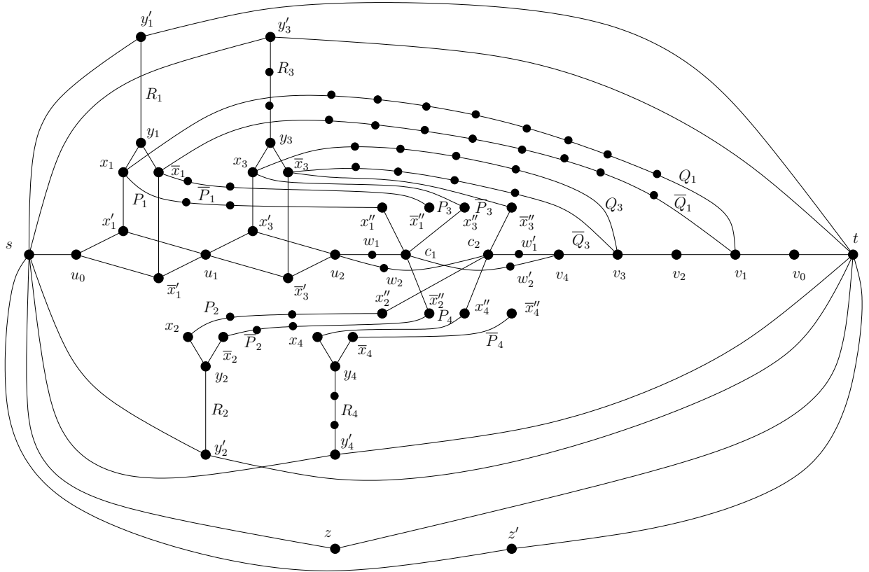
Figure 4: The construction of G for \varphi = \forall x_1 \exists x_2 \forall x_3 \exists x_4 [(x_1 \vee \bar{x}_2 \vee x_3) \wedge (x_2 \vee \bar{x}_3 \vee x_4)] .
