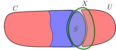
Figure 1: A visualization of the set X , the component C , the sets S , and U , and the way the red and blue colors are distributed among them.
