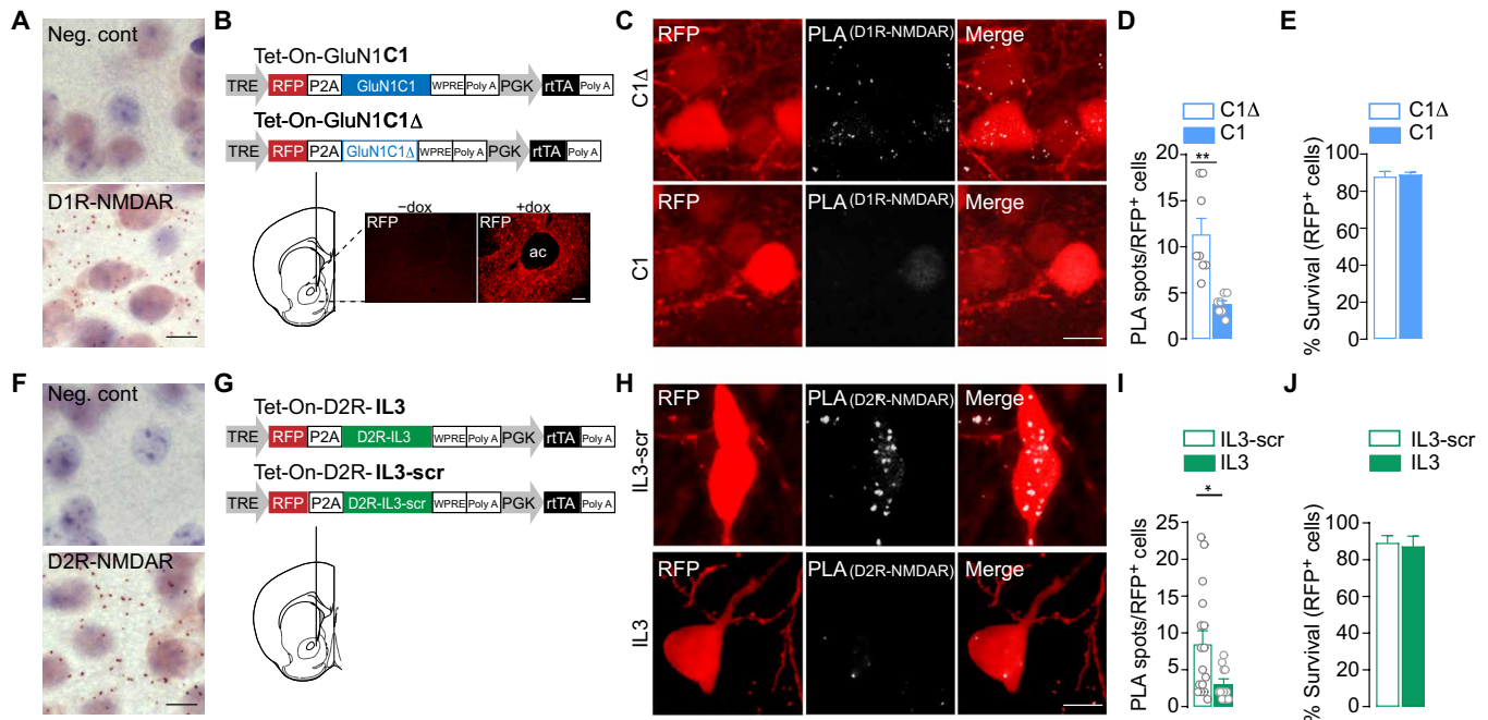
Fig. 1. Detection and temporally controlled disruption of striatal D1R-NMDAR and D2R-NMDAR heteromerization in vivo. (A) Example images of D1R-NMDAR heteromer PLA detection and related negative (Neg. cont) showing the absence of signal when one primary antibody is omitted. (B) Top: Viral-based strategy for expression of interfering peptide to disrupt D1R-NMDAR interaction [Tet-On-GluN1C1 (C1)] and control [Tet-On-GluN1C1Δ (C1Δ)] in the NAc. Bottom: Example image of dox (+dox)-mediated RFP expression [anterior commissure (ac)]. TRE, tetracycline response element; P2A, 2A peptide; PGK, phosphoglycerate kinase 1 promoter; rtTA, reverse tetracycline-controlled transactivator. (C) Example image of D1R-NMDAR heteromer detection by PLA in C1Δ- and C1-transduced neurons. (D) Quantifications of the fluorescent PLA signal in C1Δ- and C1-transduced neurons. Two-sided Student's t test, t = 4.078 , df = 13 , **P = 0.0013 , n = 7 to 8 cells from four mice per group. (E) Neuronal survival of C1Δ- and C1-transduced neurons. Two-sided Student's t test, t = 0.354 df = 6 , P = 0.735 , n = 4 mice per group. (F) Same as in (A), for D2R-NMDAR heteromer PLA detection. (G) Viral strategy for expression of interfering peptide to prevent D2R-NMDAR heteromerization [Tet-On-D2R-IL3 (IL3)] and control [Tet-On-D2R-IL3-scr (IL3-scr)]. (H) Representative image D2R-NMDAR heteromer detection by PLA in IL3-scr- and IL3-transduced neurons. (I) Quantifications of the fluorescent PLA signal in IL3-scr- and IL-3 infected neurons. Two-sided Student's t test, t = 2.393 , df = 25 , *P = 0.0246 , n = 11 to 16 cells from 4 mice per group. (J) Neuronal survival of IL3-scr- and IL3-transduced neurons. Two-sided Student's t test, t = 0.2767 df = 6 , P = 0.7913 , n = 4 mice per group. Scale bars, 10 \mu\text{m} . Error bars denote SEMs.
