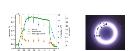
Electron density and temperature variations [10] (left) during pulsing of a planar magnetron Ar plasma at 7.5 mTorr (right)
