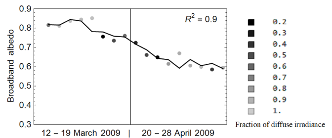
Figure 8. The relationship between the albedo values corresponding to the solar zenith angle value of 73° measured operationally at Sodankylä and the regression (albedo = 0.84 – 0.29 b – 0.008 k_0 ) based on measured surface roughness parameters b (Eq. 1) and k_0 (Eq. 2) at the NorSEN mast in March and April 2009. The darkness of the markers is related to the fraction of diffuse irradiance.
