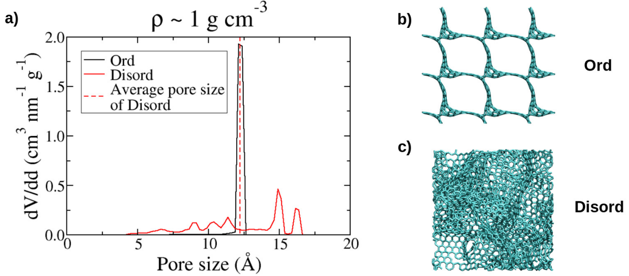
FIG. 2. a) Pore size distributions of the two porous carbon structures used in this work. b) The Ord carbon is characterized by a unimodal pore size distribution while c) the Disord carbon has a much wider pore size distribution. The pore size distributions were obtained using Poreblazer. 71
