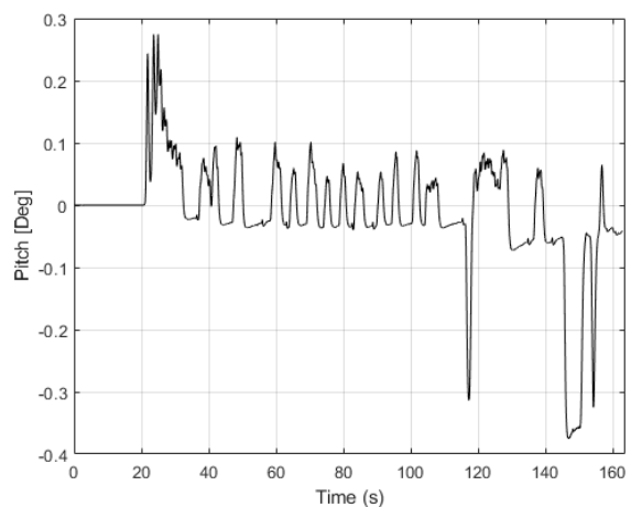
FIGURE 26. Pitch angle.
