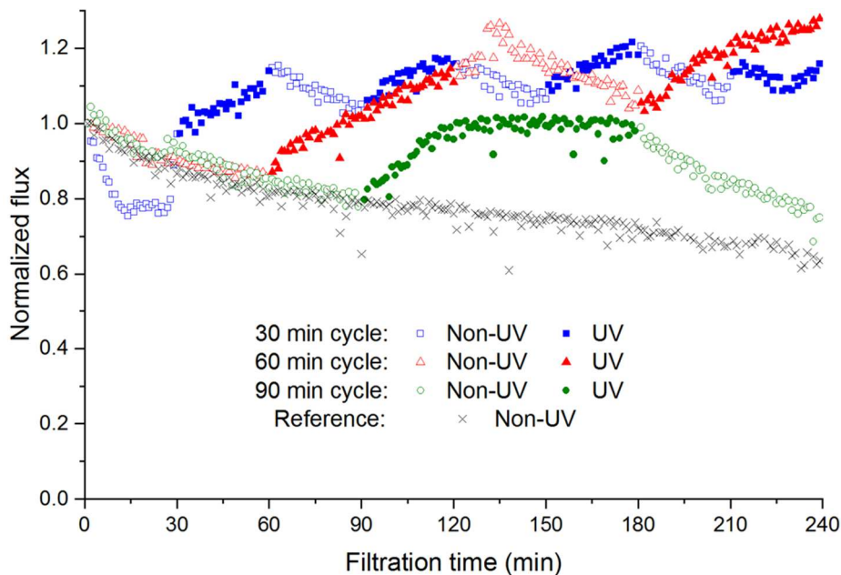
Fig. 8. Permeate flux behavior with different irradiation cycles ( I = 1 \text{ mW}\cdot\text{cm}^{-2} ).
