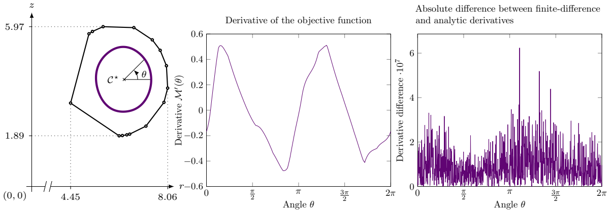
Figure 2: Numerical results on a 15-sided polygon (left) in axisymmetric. Analytic and finite-differences gradients are almost superimposed (middle). The absolute difference is about 6 \times 10^{-7} (right).
