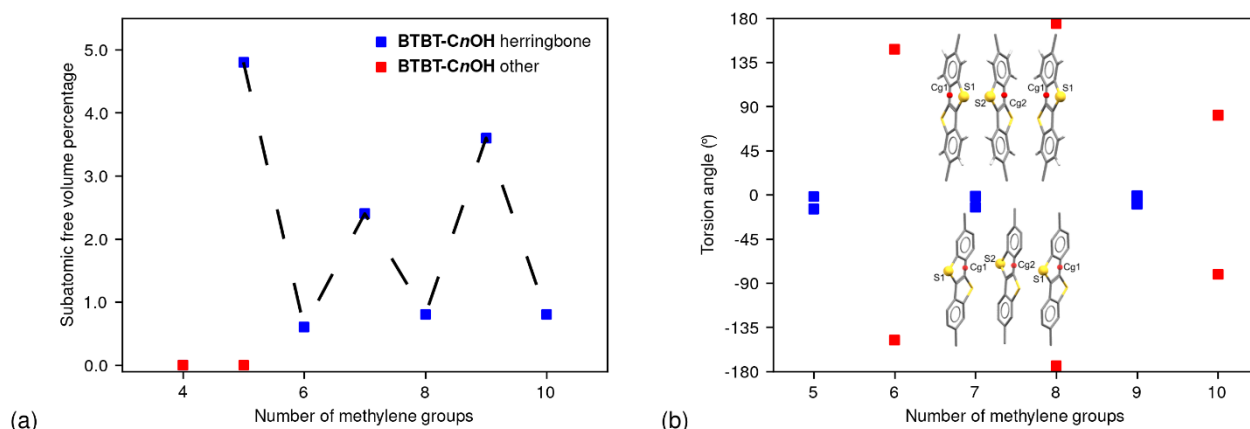
Figure 7 (a) % free volume per unit-cell volume versus number of methylene groups in BTBT- Cn OH for a probe radius of 0.95 Å and a grid-spacing of 0.1 Å. The blue points are for the structures that stack according to the herringbone mode, whereas the red points are for structures with other stackings. (b) : Torsion angles Cg1...S1...Cg2...S2 (first and second molecule from left to right) and Cg2...S2...Cg1...S1 (second and third molecule from left to right). The upper structural drawing is an example of an odd-member ( i.e. BTBT-C5OH ), whereas the lower structural drawing is an example of an even member ( i.e. BTBT-C6OH ). The lower and the upper values for the even members are dependent of each other because of space group symmetry, whereas the values for the odd members are symmetry-independent. The markers are blue for the odd members and red for the even members.
