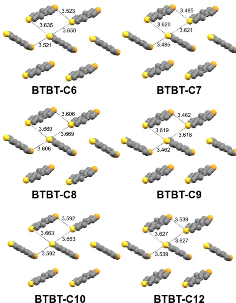
Figure 3. Projections of the BTBT-C n structures for n =6,7,8,9,10, 12 along the c -axis. It is noted that the crystal structure of the n =11 member could not be obtained. For clarity, hydrogen atoms and alkyl chains are omitted in all sub-figures. The yellow sulfur atoms are in the foreground, whereas the orange sulfur atoms are in the background. They all present the classical herringbone pattern.
