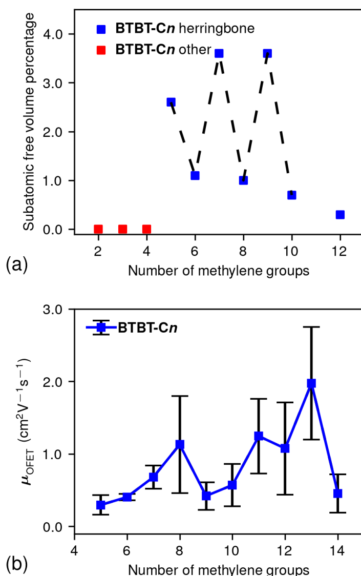
Figure 2 (a) % free volume per unit-cell volume versus number of methylene groups in BTBT- C_n for a probe radius of 0.95 Å and a grid-spacing of 0.1 Å. The blue markers are for the structures that stack according to the herringbone mode, whereas the red markers are for structures with other stackings. It is noted that the crystal structure of the n=11 member could
