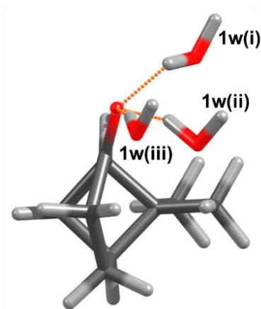
Figure 1. Illustration of the monohydrate clusters, the position of NOP is fixed to help visualization. As it shown the position of water conformers 1w(ii) and 1w(iii) is close. This fact can explain the non-convergence of some DFT methods for those structures.
