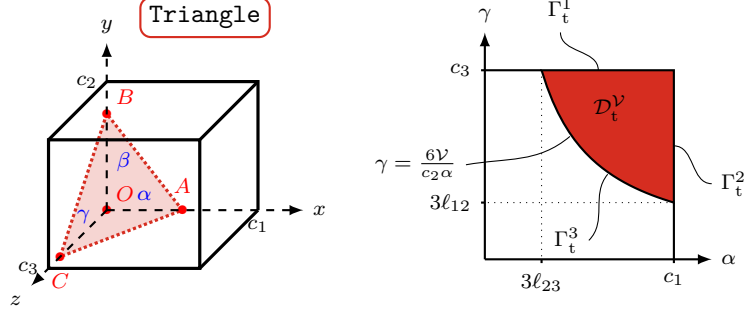
Figure C.12: Triangle configuration (left) and definition domain \mathcal{D}_t^V with \chi < \frac{1}{6} (right).
