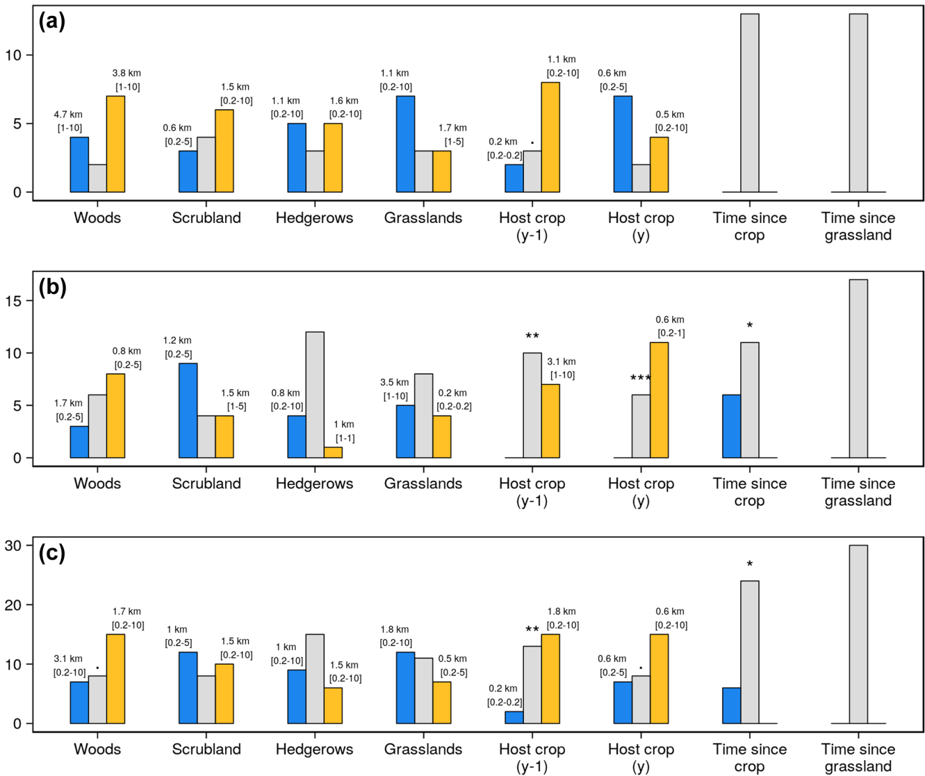
Figure 2. Number of organisms for which the risk of exceeding the abundance thresholds is correlated positively (orange), negatively (blue) and unaffected (grey) by each of the variables for (a) pests, (b) pathogens and (c) all organisms confounded (median over 1000 bootstrapped fits). Spatial variables (all but ‘time since crop’ and ‘time since grassland’) are assessed in four buffers: 200 m, 1, 5 and 10 km but only the dominant scale across replicates is accounted for. Host crop area (y) refers to the host crop area during the ongoing growing season of the observation, and (y – 1) refers to the previous growing season. Time since crop or grassland corresponds to the number of years (1, 2 or more) since the host crop or grassland was grown in the same field. The geometric average, the minimum and the maximum of the scales (buffer radii) with the highest effect size over the different organisms are indicated above the bars. p-value levels for the two-sided binomial test comparing the numbers of organisms positively and negatively correlated with a component are indicated by: ‘.’: p < 0.1 , ‘*’: p < 0.05 , ‘**’: p < 0.01 and, ‘***’: p < 0.001 .
