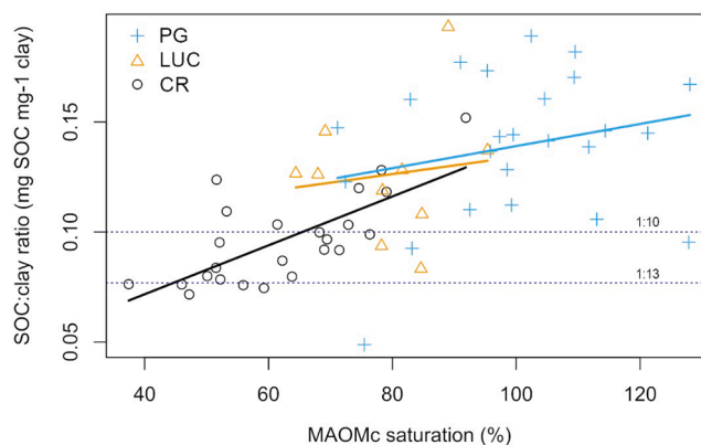
Fig. 3. Relationship between soil physical quality defined as the SOC:clay ratio and organic C saturation in the MAOM fraction in permanent grassland (PG), land-use change (LUC) and cropland (CR) sites. The thresholds for good (ratio > 0.10) and poor (ratio < 0.077) soil physical quality as defined by Johannes et al. (2019) are indicated by horizontal dotted lines. The PG site with SOC:clay ratio < 0.05 and high clay content is represented in the figure, but it is excluded from the ANCOVA analysis (n = 57).
