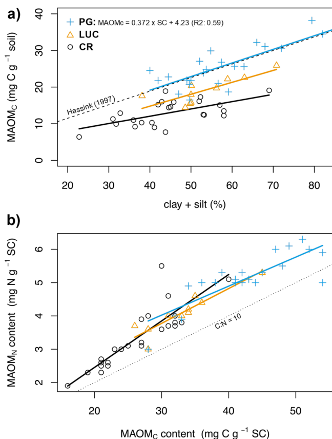
Fig. 1. Effect of land-use type on the relationships between (a) mineral-associated organic C ( \text{MAOM}_C ) and the mass proportion of silt + clay particles ( < 50 \mu\text{m} , SC) and between (b) the contents of organic C ( \text{MAOM}_C ) and total N ( \text{MAOM}_N ) in the silt + clay fraction. Solid lines represent the regression for permanent grasslands (PG), croplands (CR) and sites having experienced at least one land-use change in the last 30 years (LUC). The dashed line in (a) represents the relationship for permanent grassland found by Hassink (1997), whereas the dashed line in (b) represents the carbon to nitrogen (C:N) ratio = 10 of MAOC.
