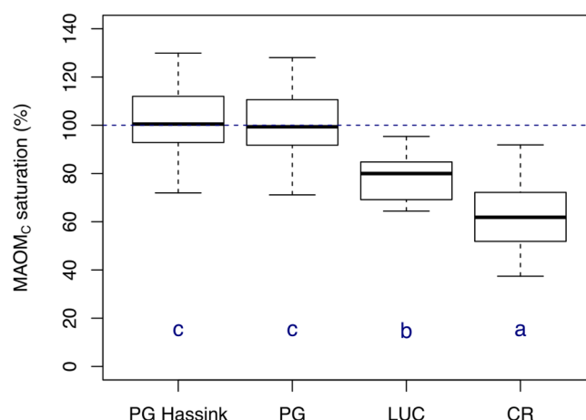
Fig. 2. \text{MAOM}_C saturation in croplands (CR) and land-use change sites (LUC) using \text{MAOM}_C in permanent grasslands (PG) as reference level for saturated soils following the equation determined in this study: \text{MAOM}_C \text{ saturated} = 0.372 \times \% \text{SC} + 4.23 (Fig. 1). PG Hassink represents the saturation level of PG calculated using the silt + clay proportion of PG and the relationship between the proportion of silt + clay particles and \text{MAOM}_C determined by Hassink (1997): \text{MAOM}_C \text{ saturated} = 0.370 \times \text{SC} + 4.09 . Letters represent significant differences at p < 0.05 modeled by ANOVA.
