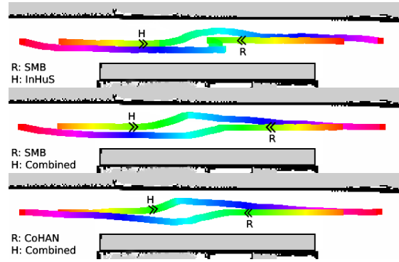
Fig. 3. Traversed paths generated by InHuS during the Narrow corridor scenario. From top to bottom the configurations are respectively : InHuS-SMB, Combined-SMB, Combined-CoHAN.
