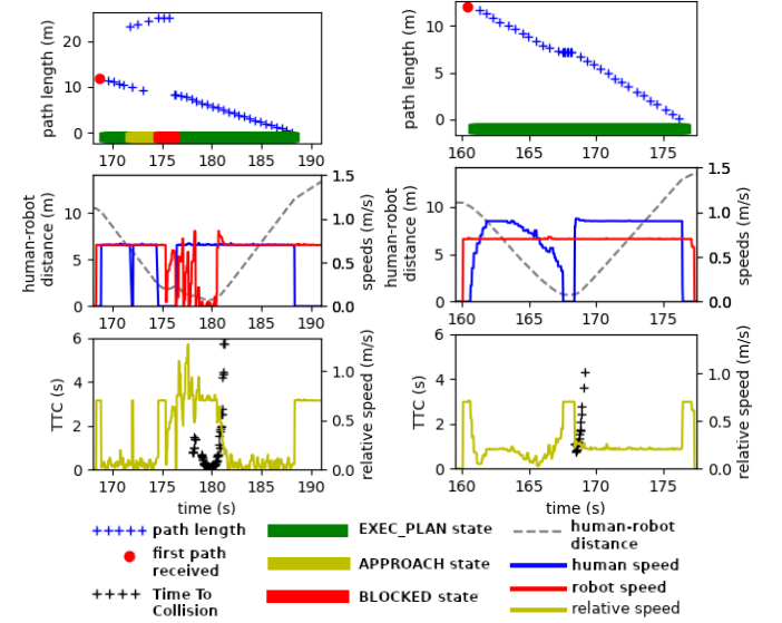
Fig. 4. Graphs of all relevant metrics recorded or computed by InHuS during the Narrow corridor scenario. The three graphs on the left are from the InHuS-SMB run and the three on the right are from the Combined-SMB run.
