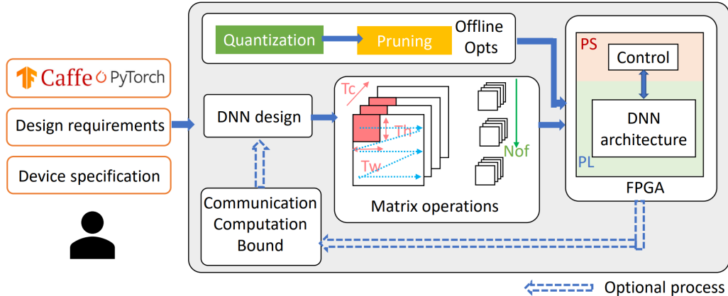
Figure 6: Generic frameworks for DNN accelerators.
