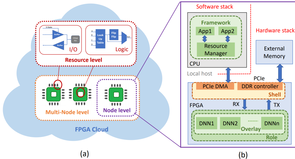
Figure 3: Overall architecture of the FPGA-based DNN accelerators in the IaaS cloud. (a) Different levels of abstraction in the FPGA virtualization technique. (b) Example of the system architecture in node-level virtualization.
