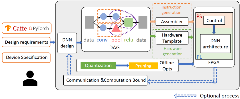
Figure 7: Generic compiler-inspired frameworks for DNN accelerators.
