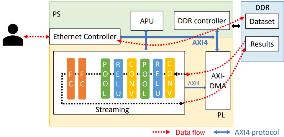
Figure 4: Example of accelerating DNNs using the streaming architecture.
