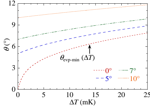
Figure 3. \theta as a function of \Delta T for different \theta_{\text{micro}} computed for pentane at 1 bar. The curve for \theta_{\text{micro}} = 0 corresponds to \theta_{\text{evp-min}}(\Delta T) .
