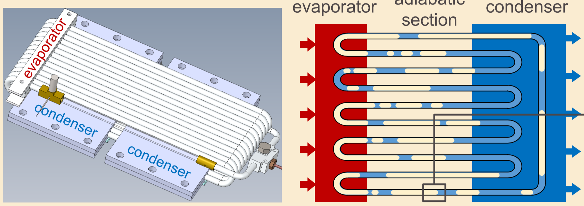
Space PHP prototype (left) and schematic (right)
