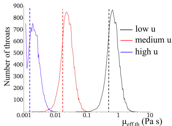
Fig. 4. Distribution of \mu_{\text{eff,th}} values for the flow of the 500 ppm polymer solution through the sand pack under different values of u . Low, medium and high u correspond to u = 1.00 \times 10^{-9} , u = 2.81 \times 10^{-6} m/s and u = 9.42 \times 10^{-4} m/s, respectively. Black, red, and blue vertical dashed lines correspond to the values of Darcy viscosity for the low, medium and high values of u , respectively. (For interpretation of the references to color in this figure legend, the reader is referred to the web version of this article.)
