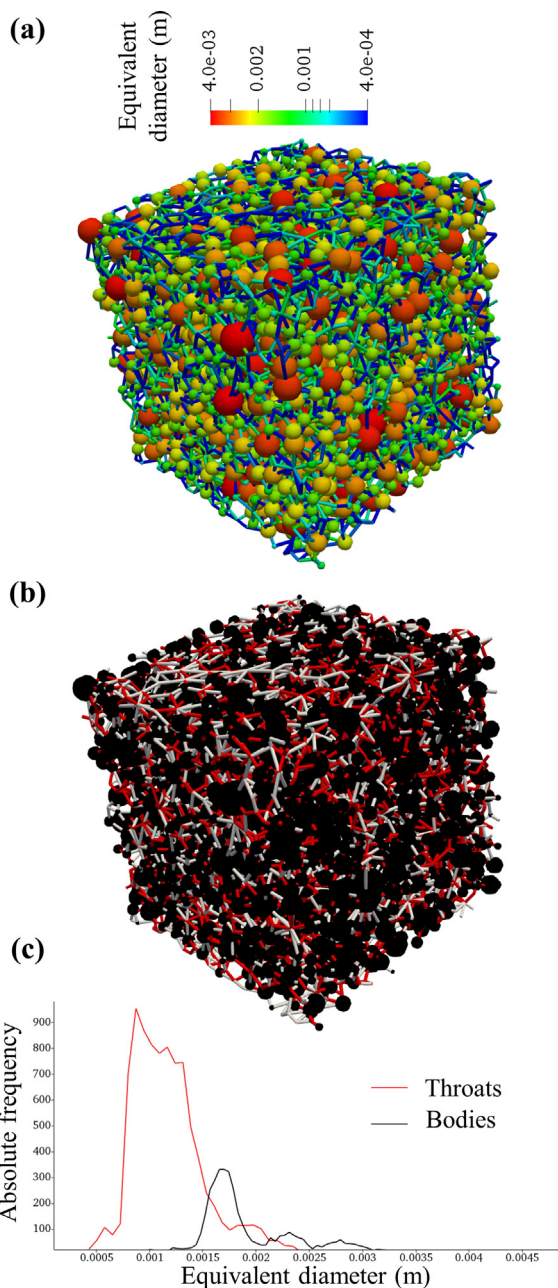
Fig. 2. Pore network model of the investigated pack of spherical beads with d_s = 4 -mm. (a) Image of the network as extracted from the 3D digital image. Warmer colors correspond to greater equivalent diameters of the pore bodies and pore throats. (b) Image representing the conducting and stagnant throats for the 700-ppm xanthan gum solution flowing at u = 3.67 \times 10^{-2} m/s. Black color represents pore bodies, red color represents conducting throats and white color represents stagnant throats. (c) Body size distribution and throat size distribution of the conducting throats. (For interpretation of the references to color in this figure legend, the reader is referred to the web version of this article.)
