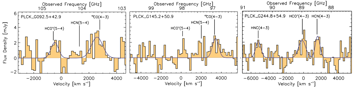
Fig. 1. Spatially integrated EMIR spectra of emission lines from high-density tracer molecules observable using a single setup in the 3-mm band. The spectra were continuum-subtracted, binned to 50\text{--}55\text{ km s}^{-1} resolution, and lines detected at >3\sigma were fitted with single Gaussian functions using the CLASS software package from GILDAS (blue curves). Additional tests were performed to confirm that these detections are real (see details in Sect. 2.1).
