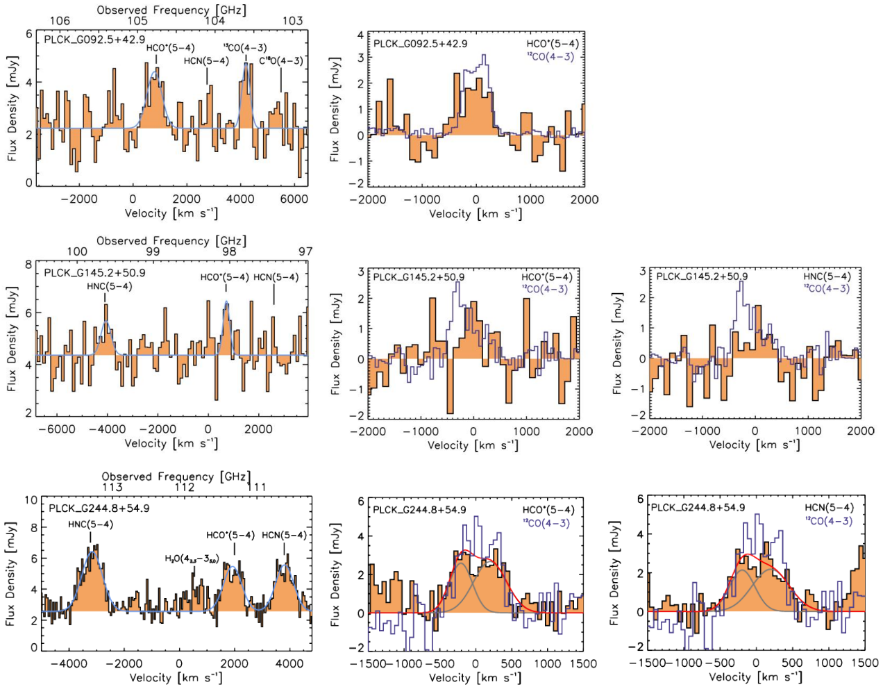
Fig. 2. Spatially integrated NOEMA spectra of emission lines from dense-gas tracers binned to 100\text{ km s}^{-1} resolution. Left: best-fit Gaussian functions obtained with the mpfit algorithm for all transitions detected at >3\sigma (blue curves), together with the continuum. Middle and right: profiles of individual lines compared with those of ^{12}\text{CO}(4\text{--}3) (blue lines). CO spectra are rescaled arbitrarily and shifted according to the best spectroscopic redshifts from C18. For PLCK_G244.8+54.9, the continuum-subtracted spectra of HCN(5–4) and HCO + (5–4) were also fitted with two Gaussian components by fixing the peak velocities to those measured for CO lines (C18). The best-fit line profiles are plotted as red curves and individual spectral components are overlaid as gray curves.
