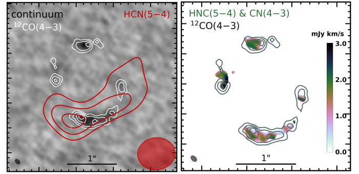
Fig. 3. Left: velocity-integrated HCN(5–4) map of PLCK_G244.8+54.9 from ALMA (red contours) with a beamsize of 0.78'' \times 0.67'' at \text{PA} = -83.6^\circ (red ellipse in the lower-right corner), compared with the CO(4–3) line emission (white contours) and 3-mm dust emission (grey background) at 0.1'' resolution from C17a. Contour levels are 4\sigma , 6\sigma , 8\sigma (red) and 3\sigma , 6\sigma , 9\sigma (white). Right: zoom onto the morphology of the velocity-integrated HNC(5–4) line emission blended with CN(4–3) (see Sect. 3.3). The black contours correspond to the white ones in the left panel. Local velocity-integrated flux densities of the blended HNC(5–4) line are shown as a color map, with the same beamsize of 0.119'' \times 0.081'' as CO(4–3) (grey ellipse in the lower-left corner).
