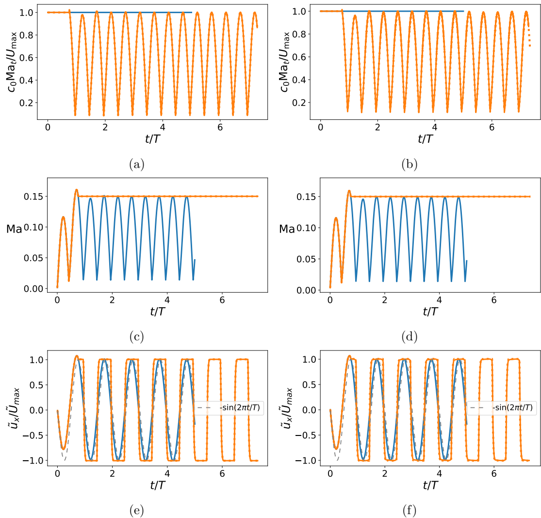
Figure 10: Temporal evolution of non-dimensional parameters related to the adaptive time-stepping for the Womersley flow. The target Mach number is \text{Ma}_t = 0.15 . Recall that U_{\max} is the (constant) overall maximum velocity and u_x(t) refers to the probed velocity at the center of the oscillating flow. The Mach number is \text{Ma} = u_{\max}(t)/c_0 when c_0 is the speed of sound. Left column : body-force stirring; Right column : inlet/outlet density conditions. (—): constant time-step; (.....): ATS; (—): ATS with correction.
