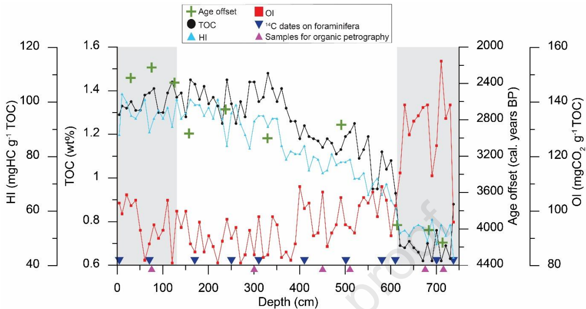
Figure 3: Hydrogen Index (HI), TOC, age offset between bulk organic matter 14 C dates and the age model based on 14 C dates of mainly benthic foraminifera (dark blue triangles), intervals sampled for organic petrography (purple triangles) and Oxygen Index (OI) plotted against core depth of the marine sediment core AMD14-204C. The grey and white boxes illustrate the three-part division of the record.
