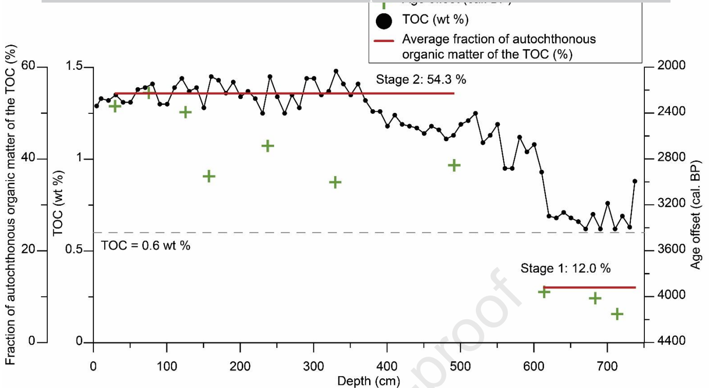
Figure 7: TOC (wt%), age offset (cal. BP) and estimated average fraction autochthonous marine algal produced organic matter of the TOC (%) for the two stages plotted against core depth.
