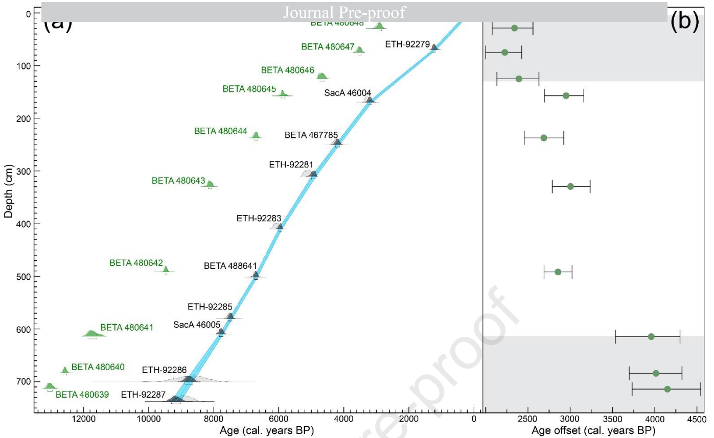
140 Figure 2: (a) Age-depth model of the marine sediment core AMD14-204C, based on mainly mixed benthic foraminifera (grey age distributions; the light shaded area for each radiocarbon date illustrate the probability distribution before age modelling, while the darker gray areas represent the probability distribution after the age model). The modeled age is shown in blue, with the envelope representing the modelled 1\sigma range (Hansen et al., 2020). The bulk organic matter dates are plotted in green (Giraudeau et al., 2020). (b) Age offsets between median calibrated bulk dates and the corresponding modelled age for each depth interval with 2\sigma uncertainties, calculated based on the 2\sigma age ranges derived from the age modelling. The grey and white boxes illustrate the three-part division of the record. 145
