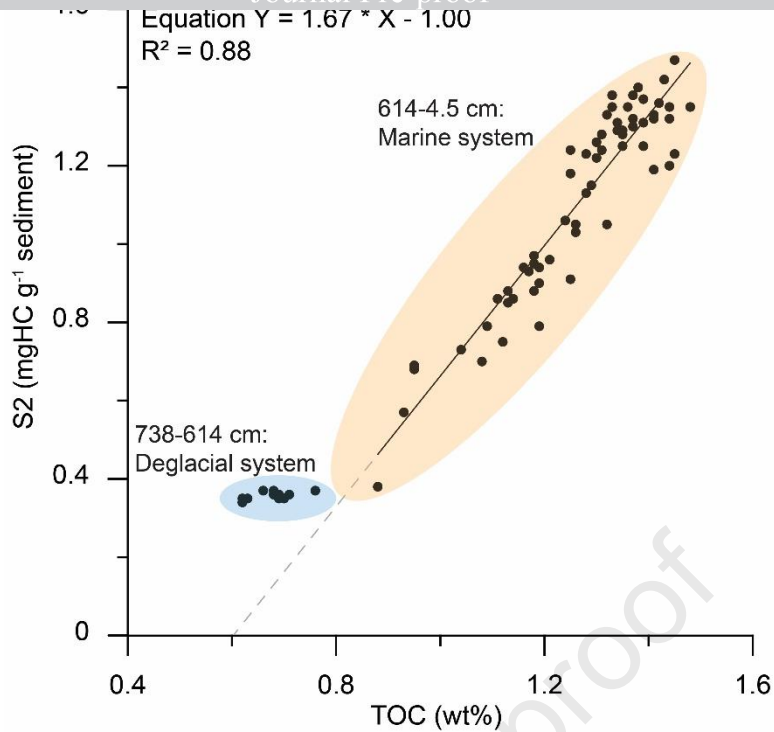
480 Figure 6: The linear correlation between the S2 and TOC in the marine system shows that the regression line intercepts at 0.6 wt% TOC.
