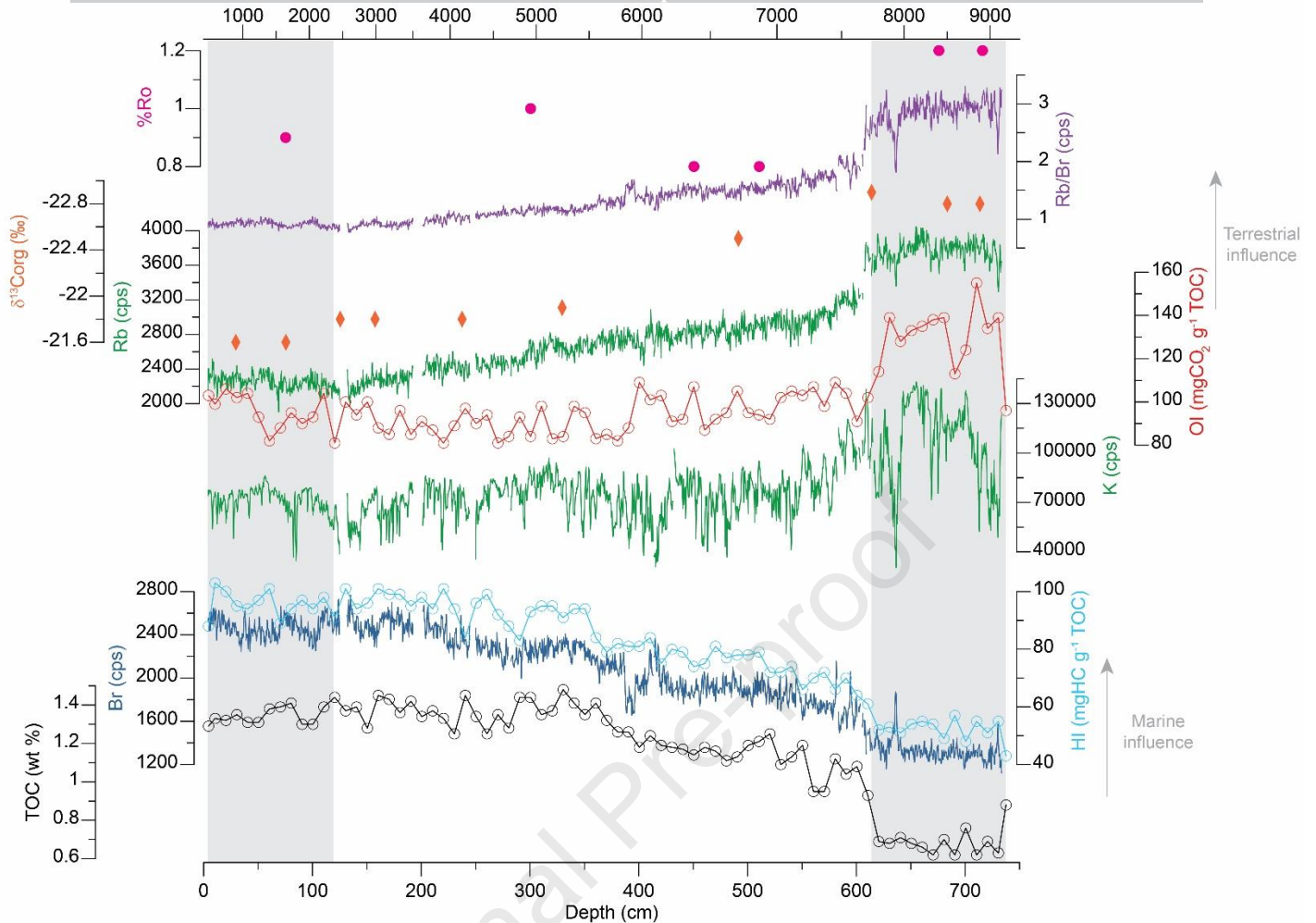
270 Figure 4: Comparison of organic pyrolysis parameters, the median %Ro, organic \delta^{13}\text{C} and X-ray Fluorescence data of core AMD14-204C. The grey and white boxes illustrate the three-part division of the record.
