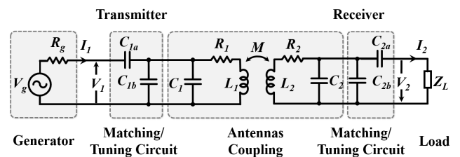
FIGURE 5. Model of an inductive power transfer (IPT) system.
