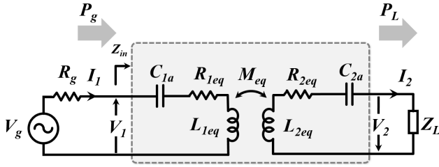
FIGURE 6. Rearranged model of an IPT System, where parasitic capacitances from coils antennas are integrated into the equivalent resistances and inductances.
