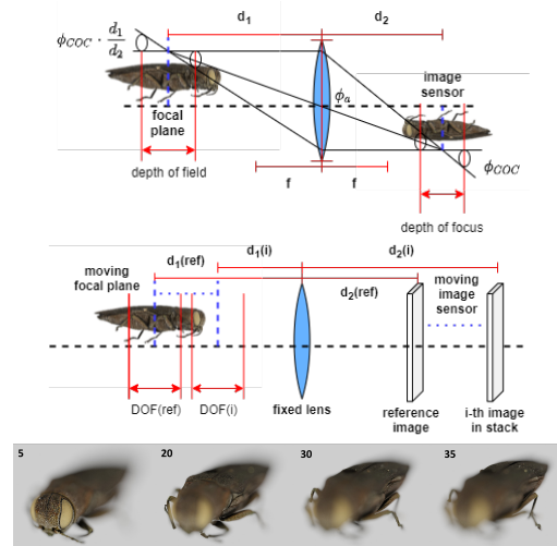
Figure 1: Top: lens image formation and circle of confusion. Middle: multi-focus capture with fixed lens setup. Bottom: example images from one stack of 61 images.
