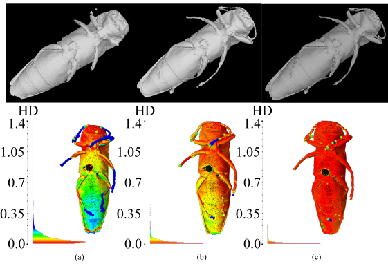
Figure 4: Reconstruction result using stacked images (top row) from different alignment methods and their Hausdorff distance to ground truth model (bottom row). (a) ECC affine with calibration target. (b) Linearly fitted ECC affine with calibration target. (c) Lens equation. Using estimated poses.
