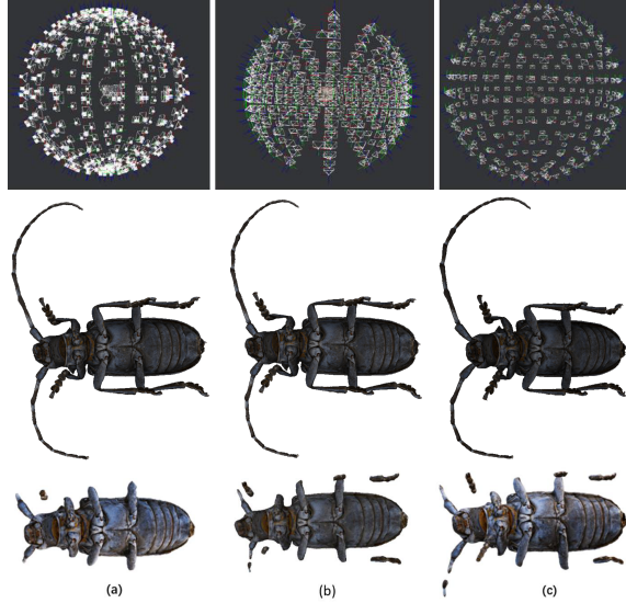
Figure 5: Effect of different pose distributions for image capture: a) constant pan-tilt rotation steps (217 poses), b) linear variation along z axis (189 poses), and c) linear variation with tilt angle (217 poses). From top row to bottom row: camera control diagram, estimated camera poses, corresponding MVS reconstructed meshes using 4320 \times 2880 pixel and 1920 \times 1080 pixel images.
