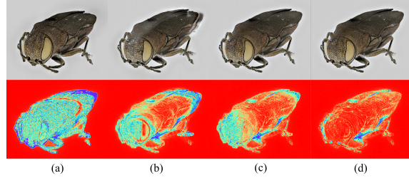
Figure 3: Focus stacked images and error maps. (a) ECC affine w/o calibration target. (b) & (c) ECC affine with calibration target and its linear fitting. (d) Lens equation.
