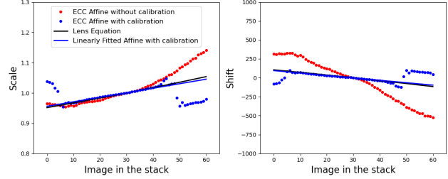
Figure 2: Distributions of the scale and shift in homography matrices estimated using different alignment methods.
