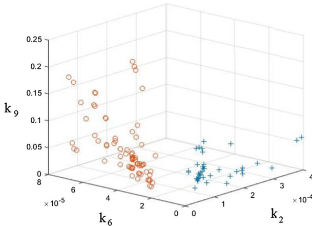
Fig. 4 Normal and hemophilic subjects are separated in the parameter space (k_2, k_6, k_9) characterizing thrombin generation curves in the case of platelet poor plasma. Hemophilic patients are shown by circles, healthy subjects by crosses. Reprinted with permission from Ratto et al. (2020a)
